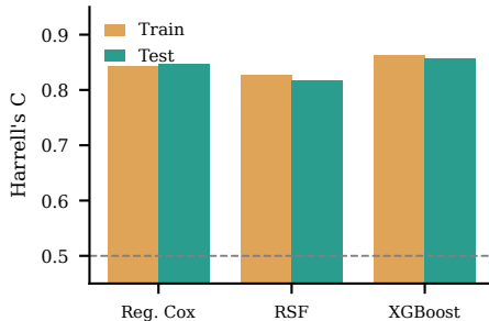
(b) Overfitting check
