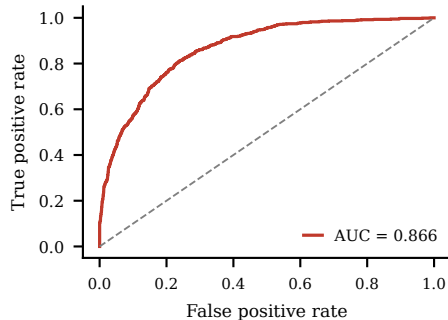
(c) Predicting who is censored
