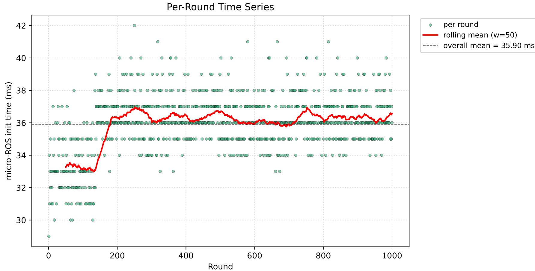
micro-ROS Entities Init Time (pico_20260619_092136.log)
