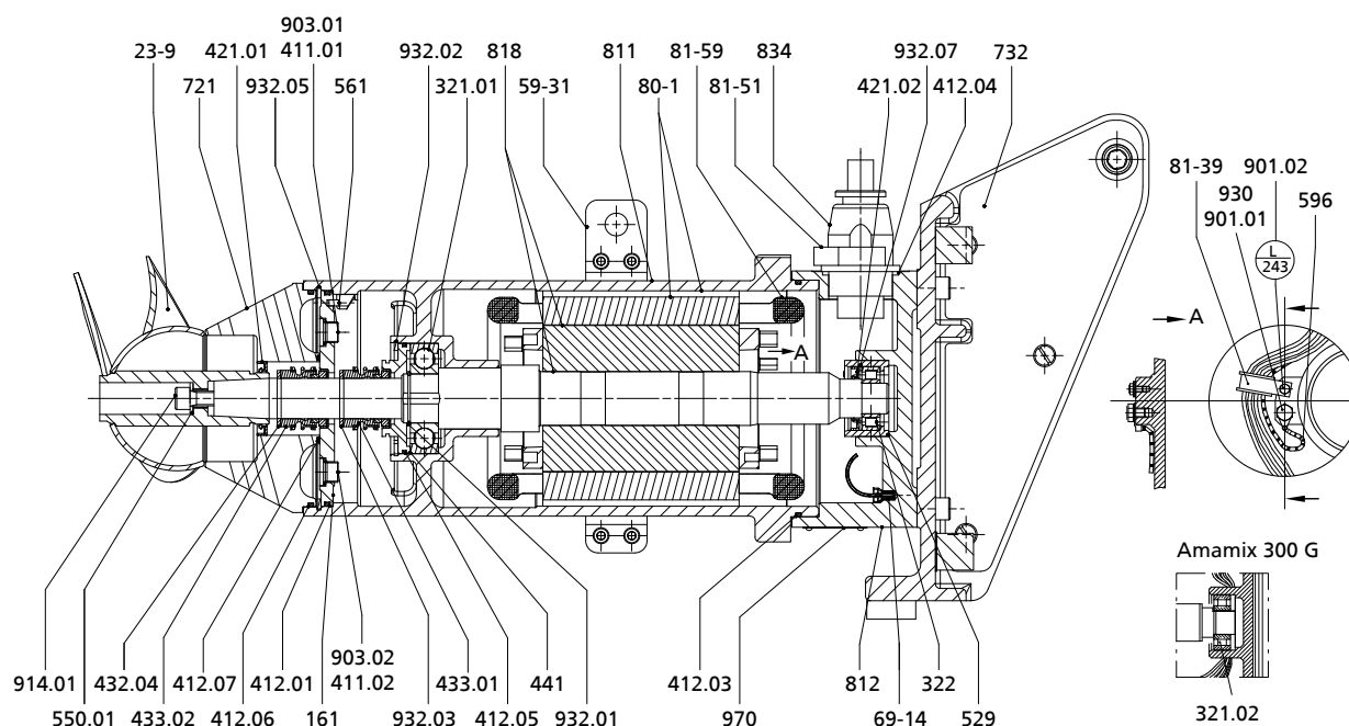
General assembly drawing Amamix 300/400/600, motor housing material gray cast iron
