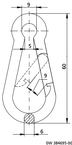
Dimensions of carabiner [mm]
