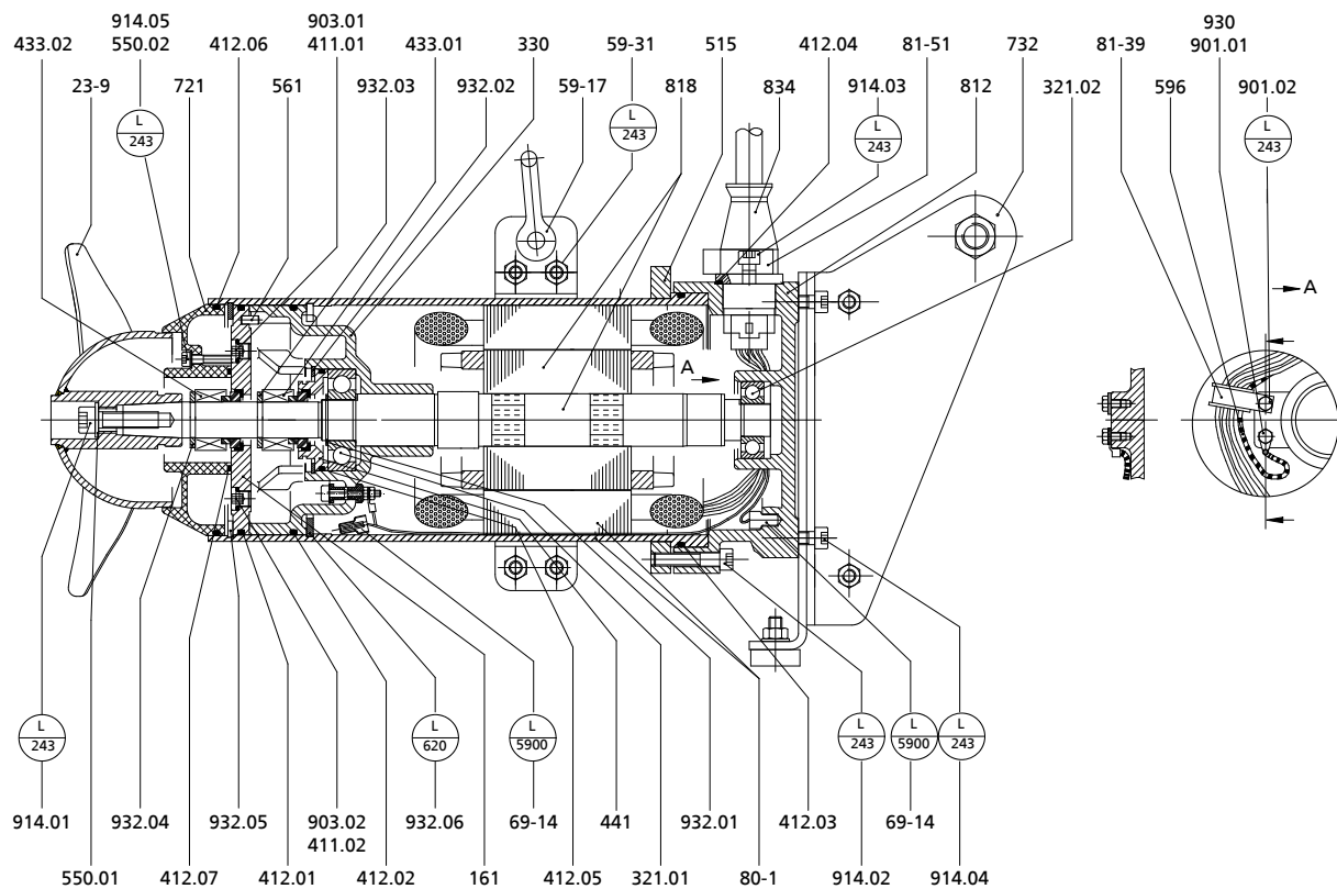
General assembly drawing Amamix 200, motor housing material stainless steel
