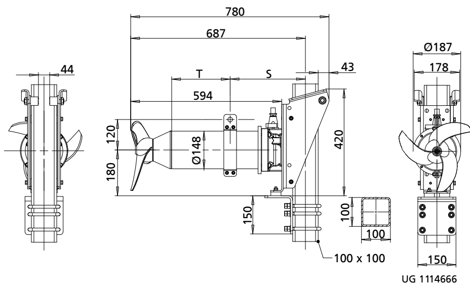
Amamix 300 C: S = 265 / T = 260, motor 0 6 / 2 6 = 48.5 kg
