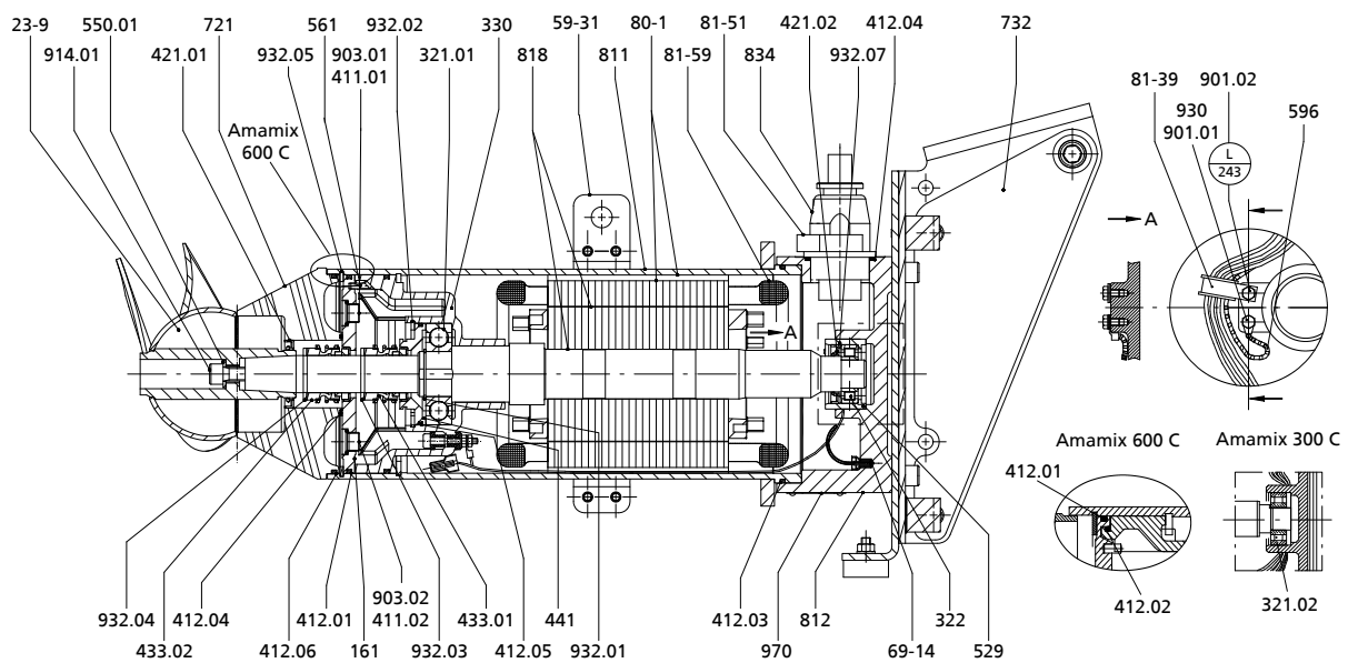
General assembly drawing Amamix 300/400/600, motor housing material stainless steel
