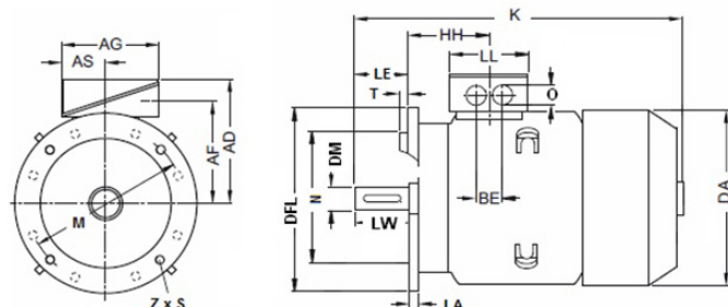
Fig. 22: Envelope dimensions
