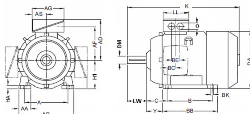
Fig. 2: Envelope dimensions
