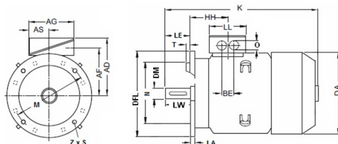
Fig. 28: Envelope dimensions
