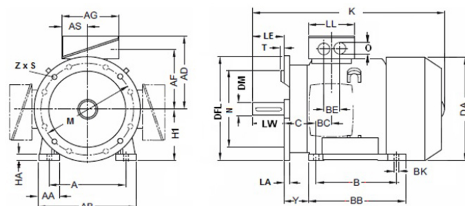
Fig. 42: Envelope dimensions
