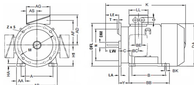
Fig. 40: Envelope dimensions
