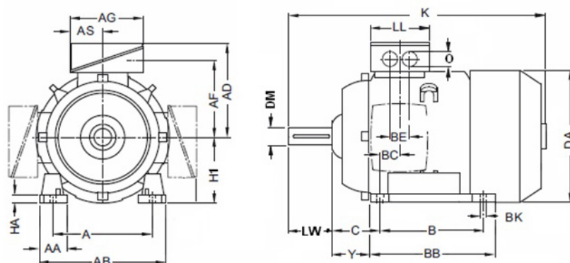
Fig. 13: Envelope dimensions
