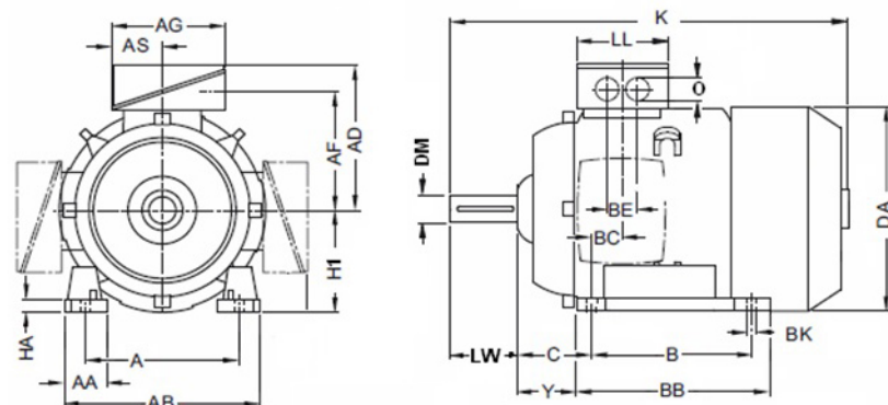
Fig. 14: Envelope dimensions
