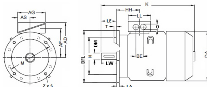
Fig. 26: Envelope dimensions
