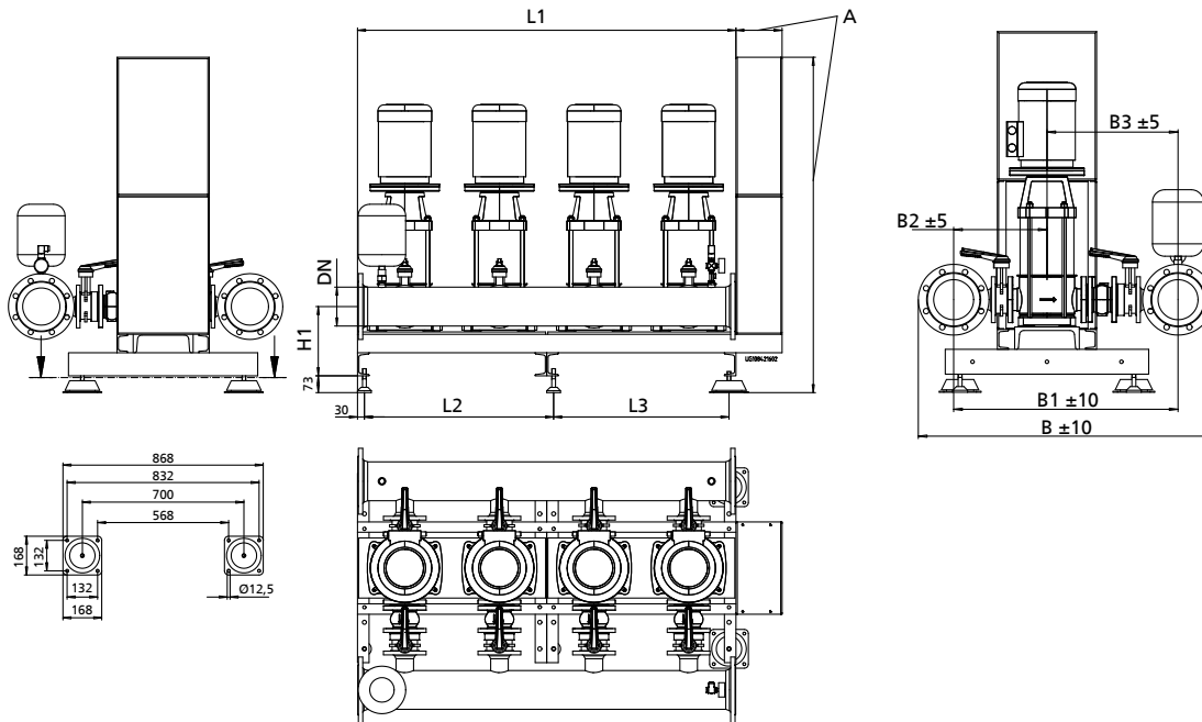
Dimensions of Hyamat V with Movitec 25B, 45, 65 and 90B
