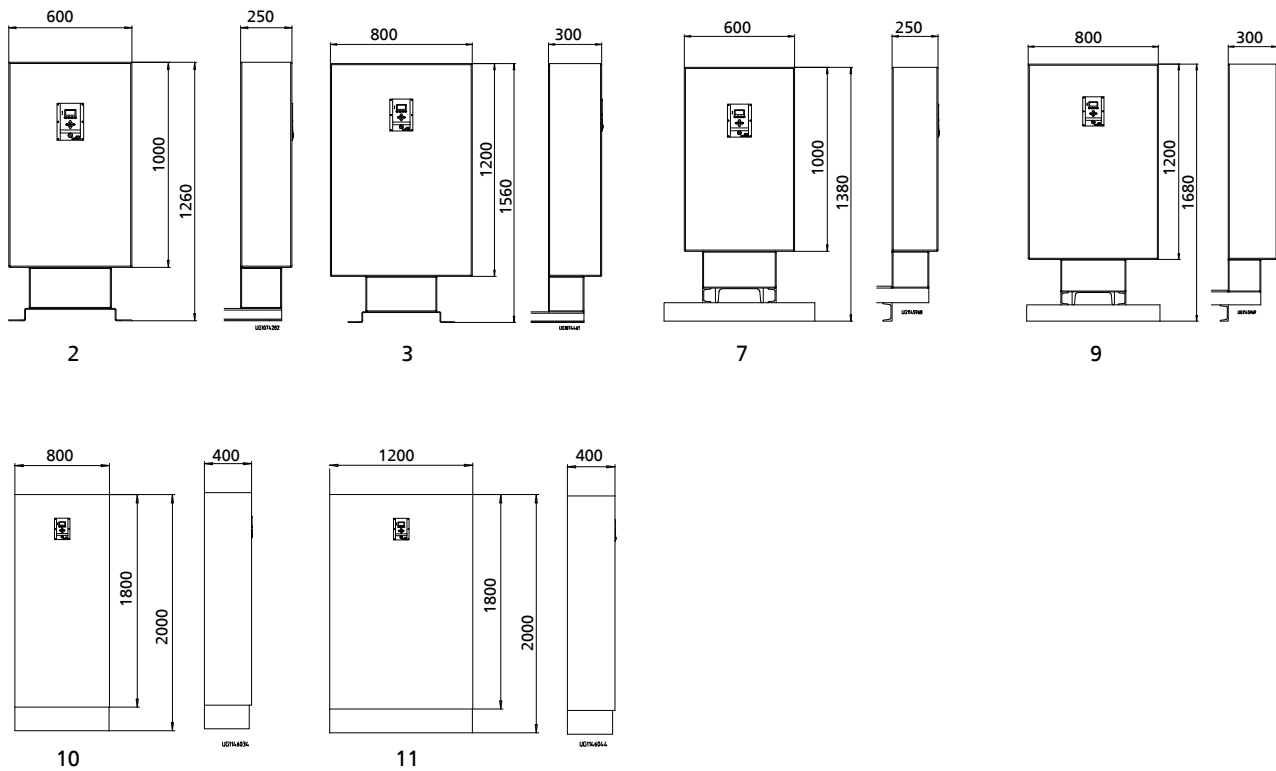
Dimensions of Hyamat V control cabinets
