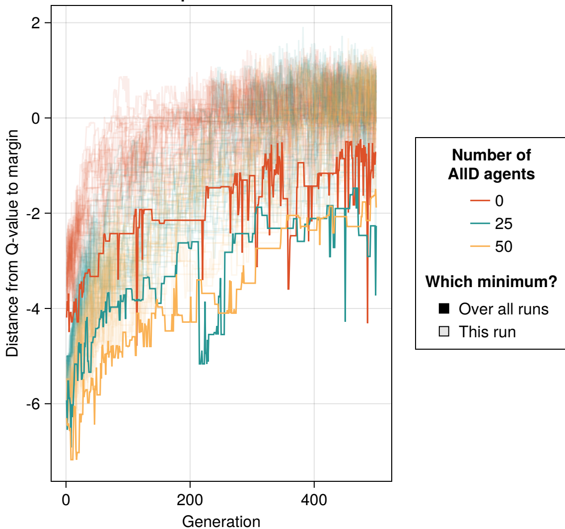
Minimum L1 distance between Q-values and line x=y for multiple runs: Norm-150
