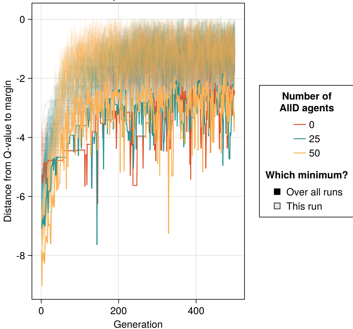
Minimum L1 distance between Q-values and line x=y for multiple runs: Norm-192
