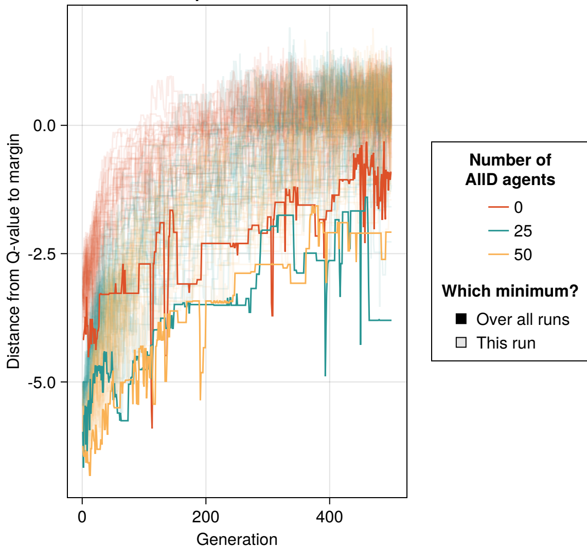
Minimum L1 distance between Q-values and line x=y for multiple runs: Norm-195
