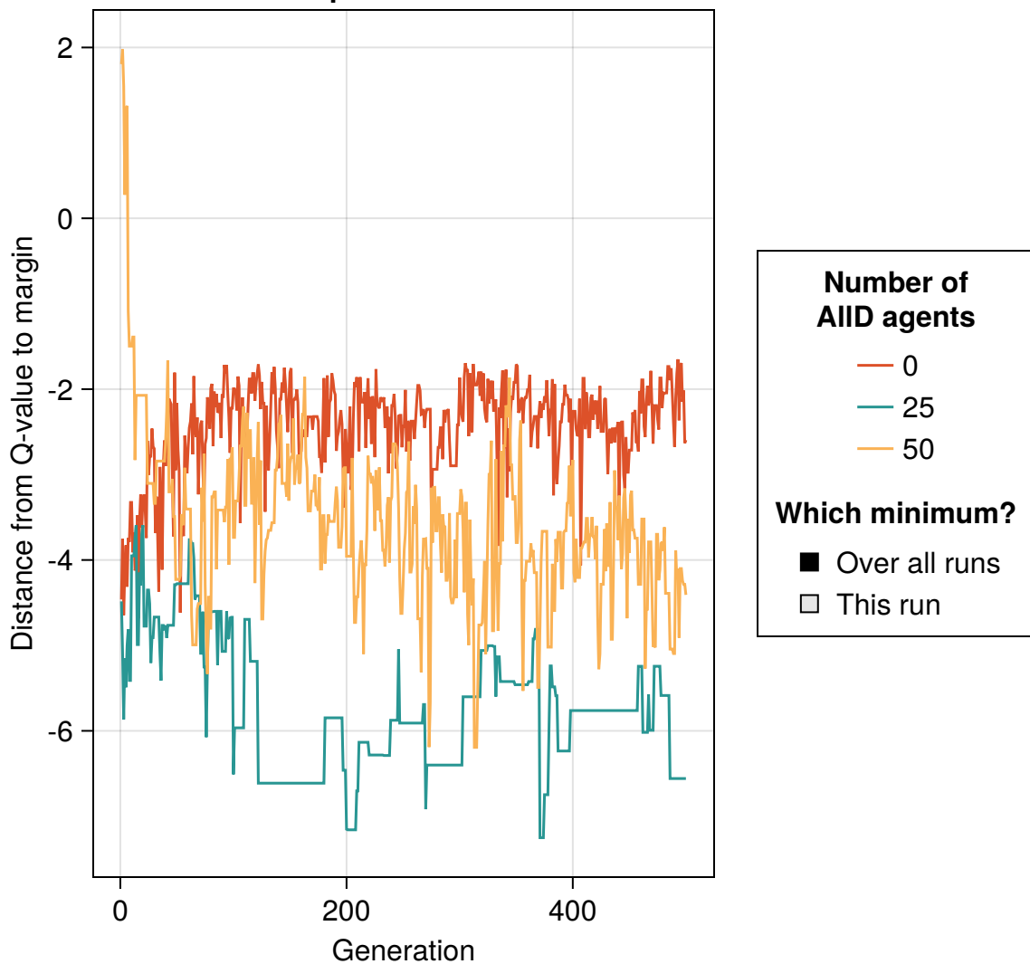
Minimum L1 distance between Q-values and line x=y for multiple runs: Norm-243
