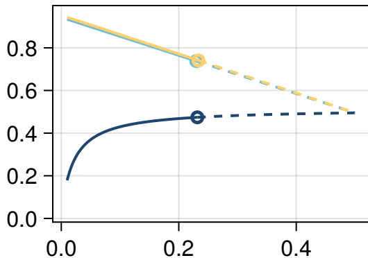
Judge execution
