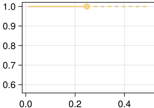
Judge execution
