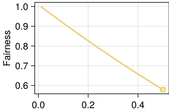
Player execution
