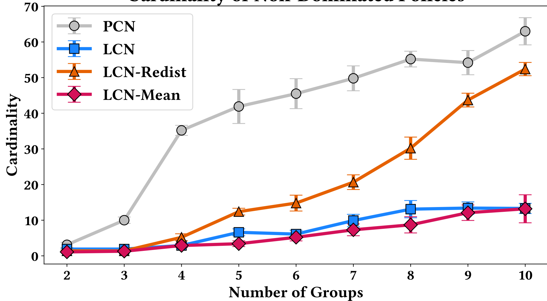
Cardinality of Non-Dominated Policies
