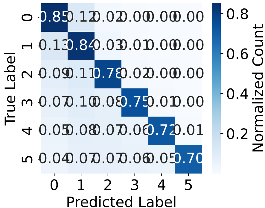
PIL Transformer
