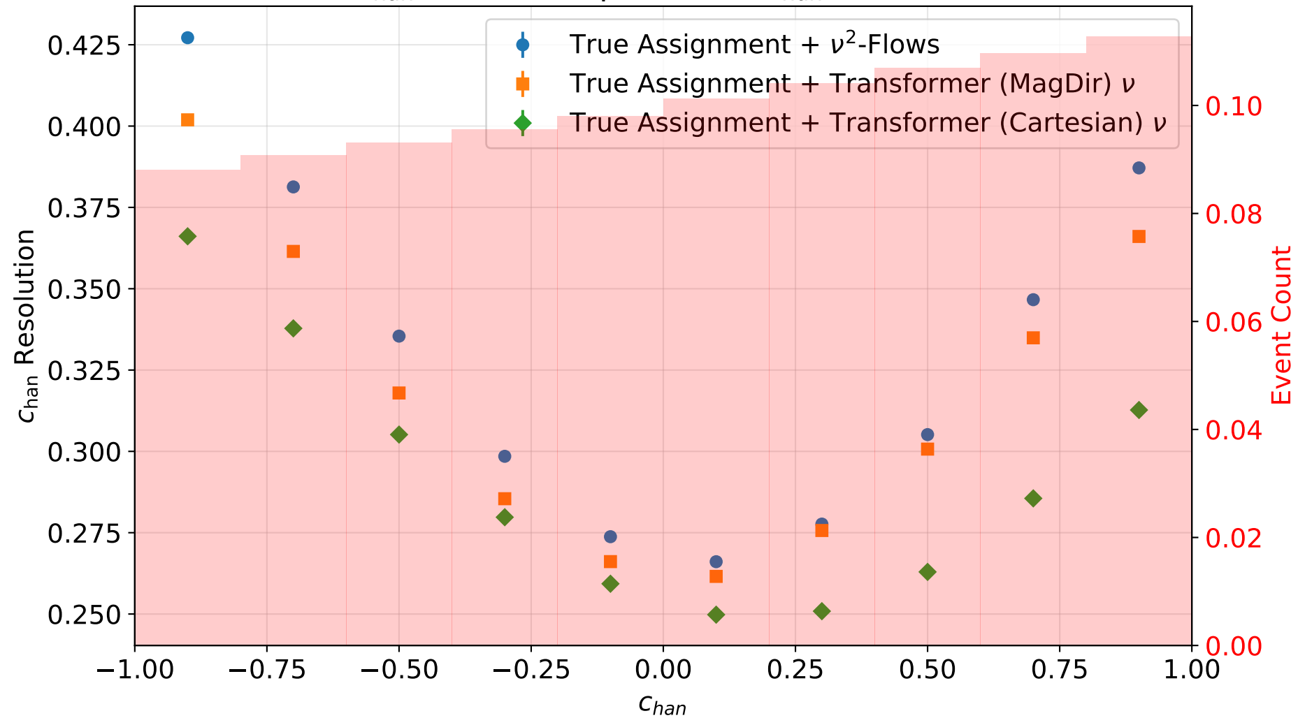
c_{chan} Resolution per Bin vs c_{chan} (95% CI)
