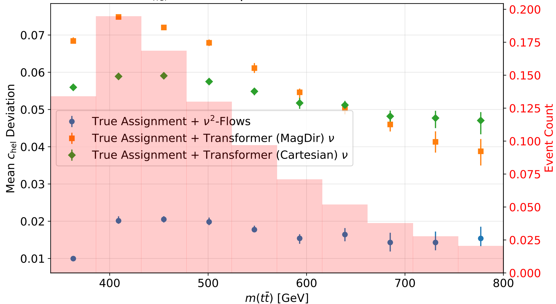
Mean c_{\text{hel}} Deviation per Bin vs m(t\bar{t}) [GeV] (95% CI)
