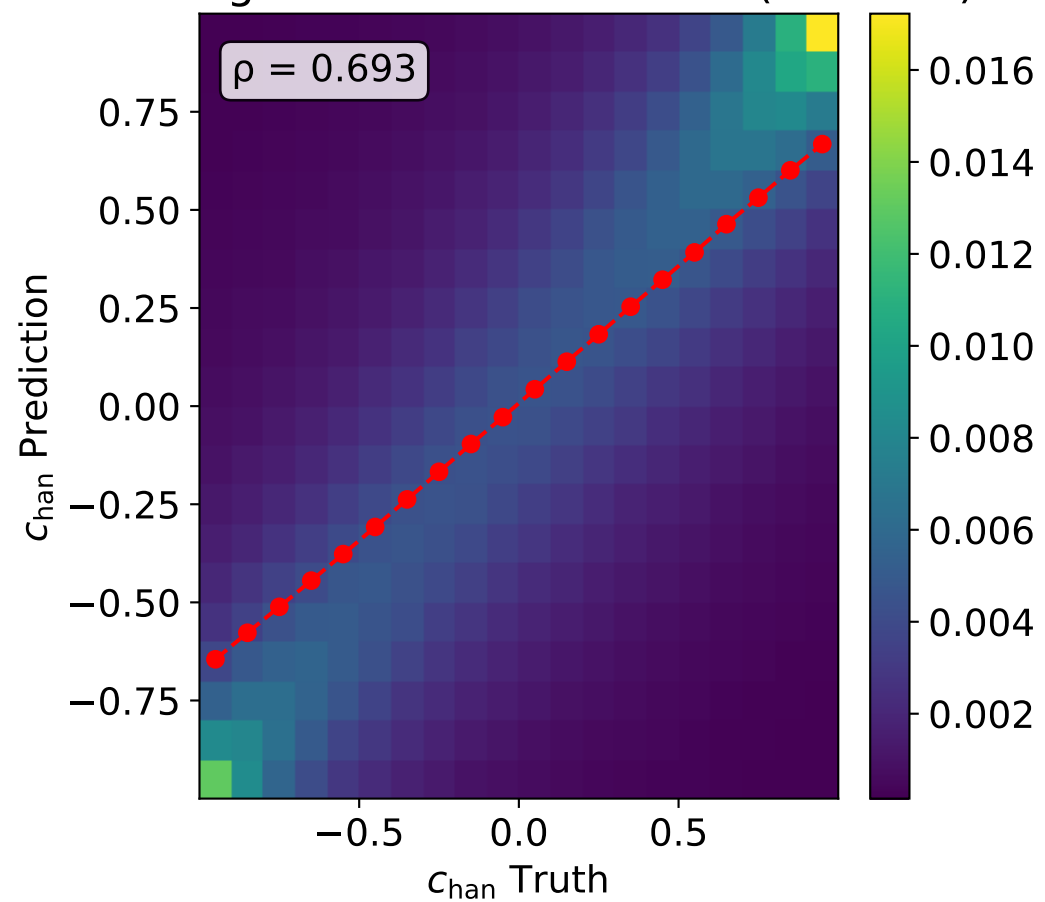
True Assignment + Transformer (PtEtaPhi) \nu
