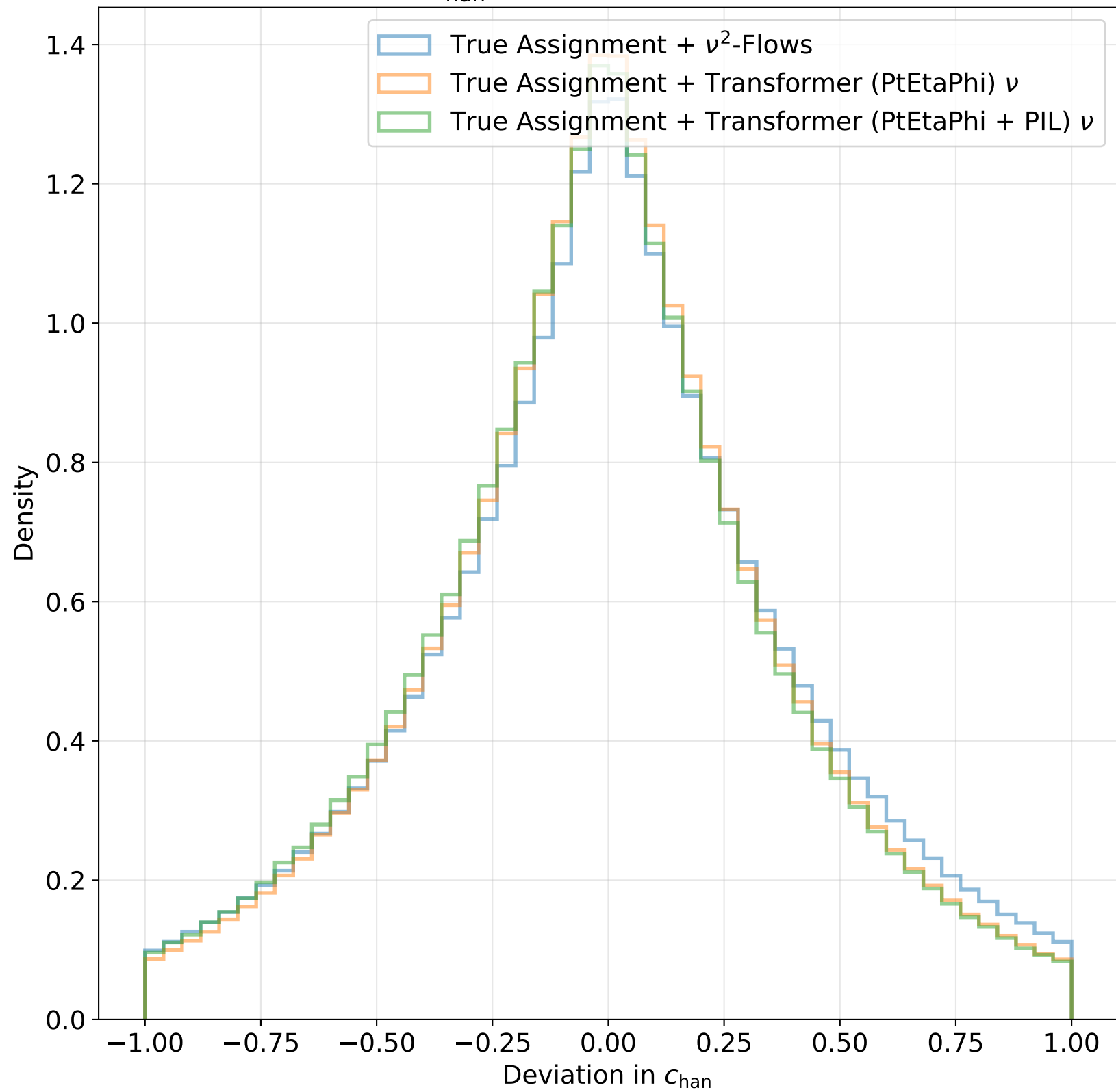
Deviation in c_{\text{chan}} Deviation for all Reconstructors
