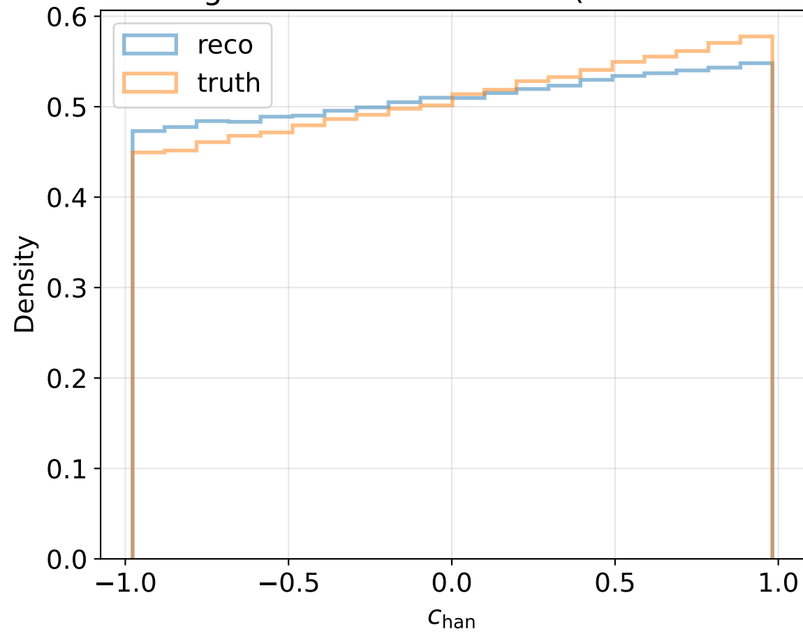
True Assignment + Transformer (PtEtaPhi + PIL) \nu
