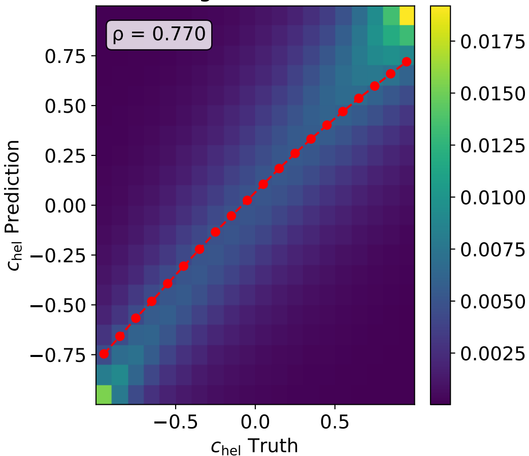
True Assignment + Transformer (PtEtaPhi + PIL) \nu
