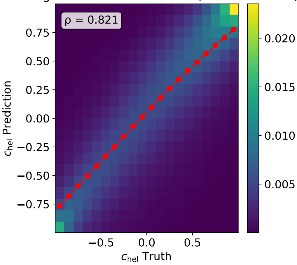
True Assignment + Transformer (PtEtaPhi + PIL) \nu
