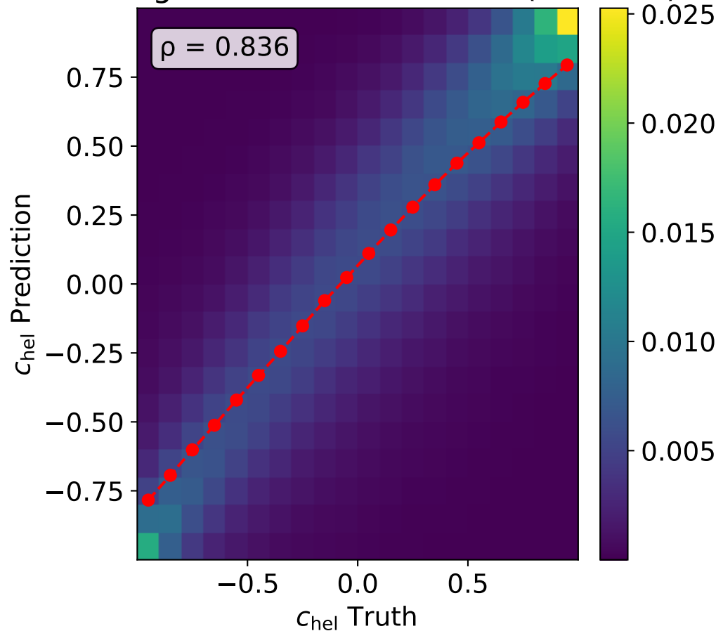
True Assignment + Transformer (PtEtaPhi) \nu
