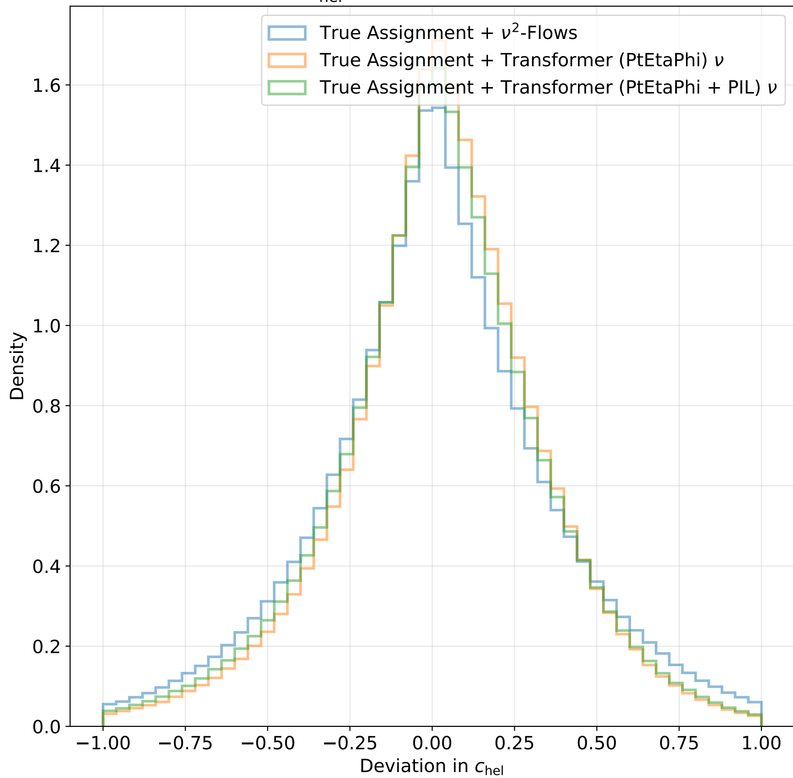
Deviation in c_{hel} Deviation for all Reconstructors
