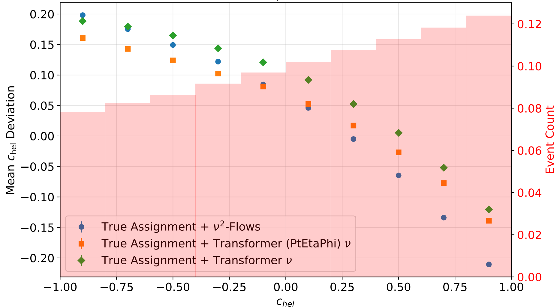
Mean c_{hel} Deviation per Bin vs c_{hel} (95% CI)
