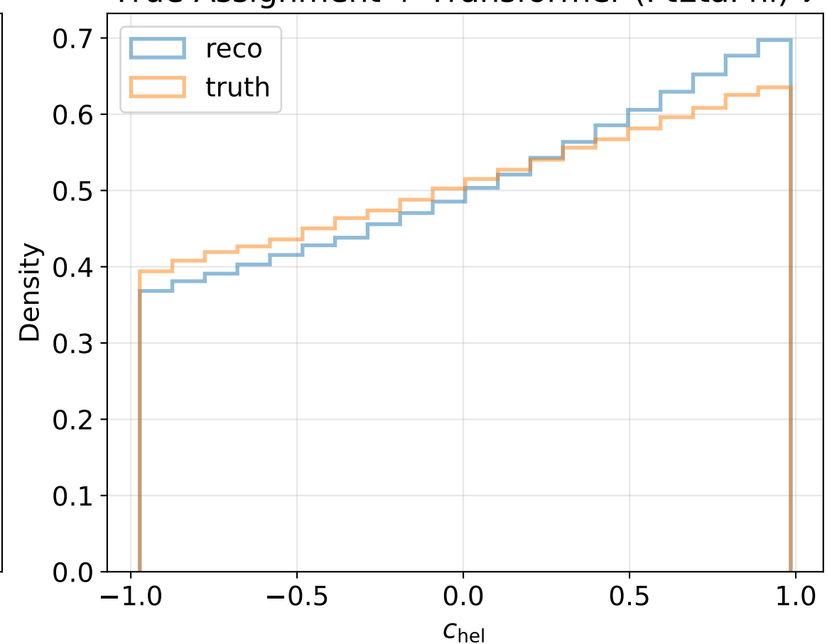
True Assignment + Transformer (PtEtaPhi) \nu
