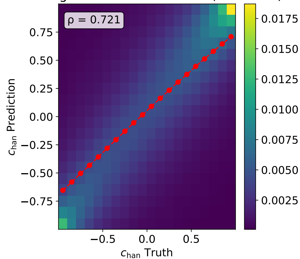
True Assignment + Transformer (Cartesian) \nu
