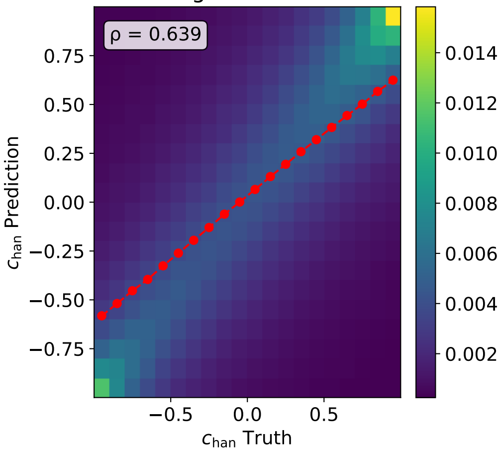
True Assignment + Transformer (Cartesian + PIL) \nu
