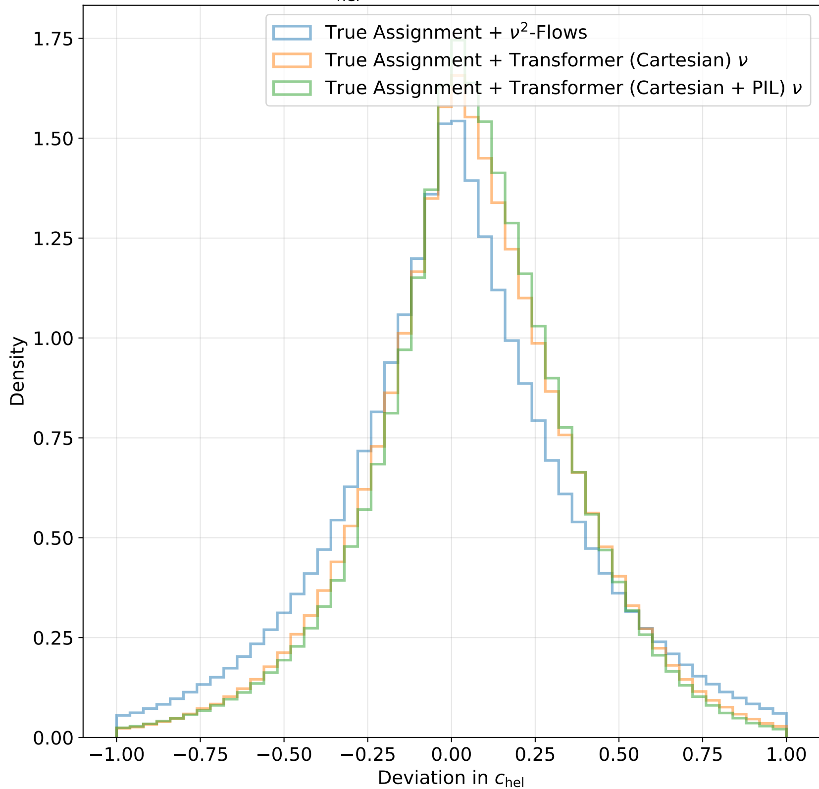
Deviation in c_{\text{hel}} Deviation for all Reconstructors
