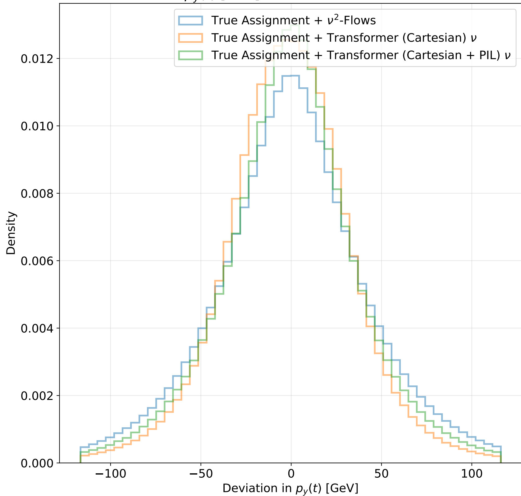
Deviation in p_y(t) [GeV] Deviation for all Reconstructors
