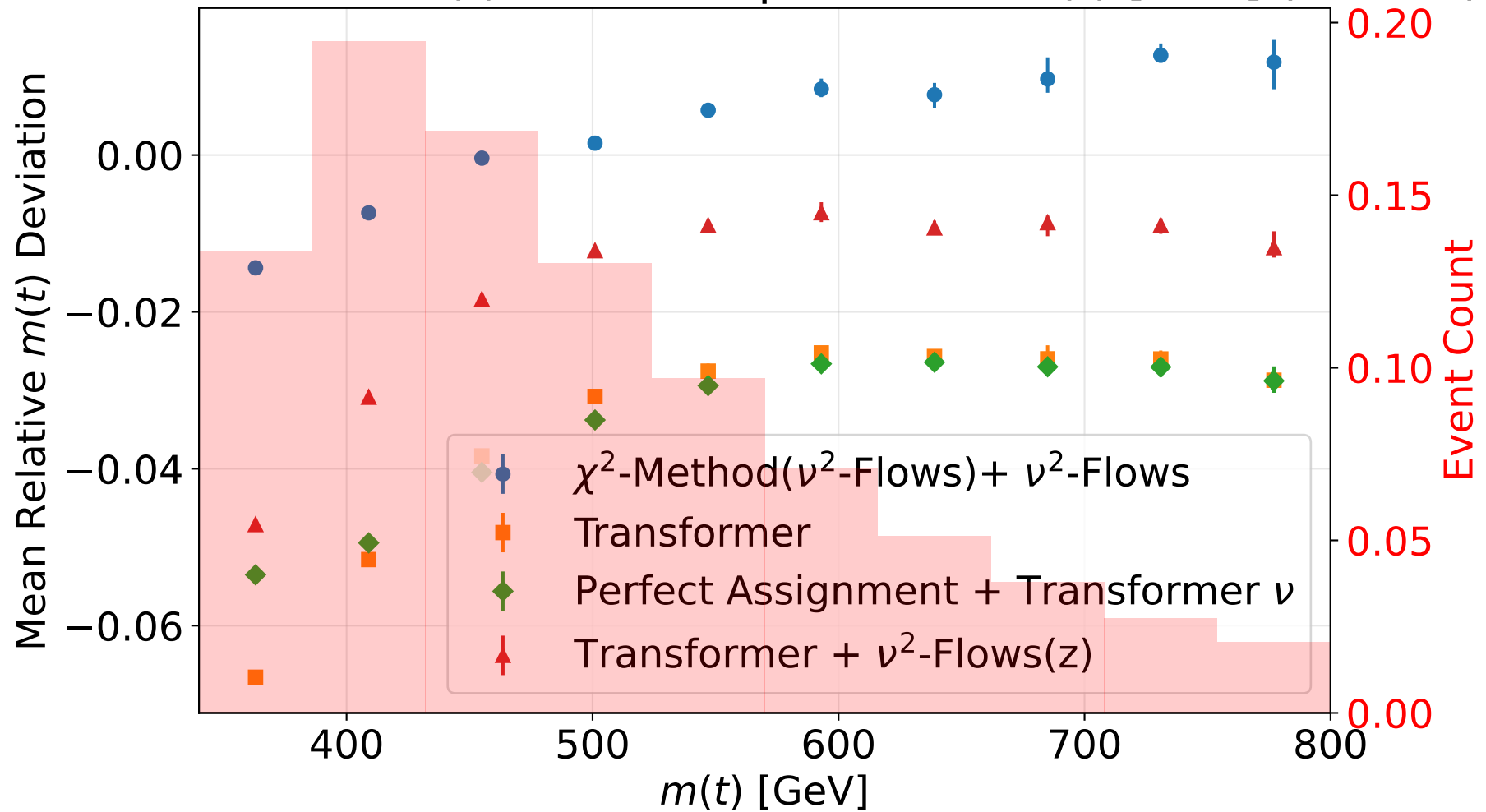
Mean Relative m(t) Deviation per Bin vs m(t) [GeV] (95% CI)
