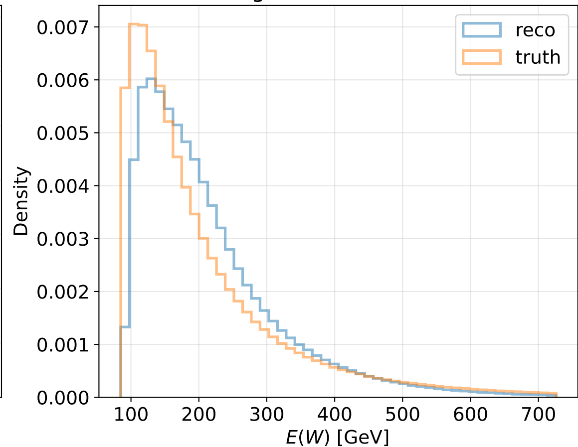
True Assignment + Transformer \nu
