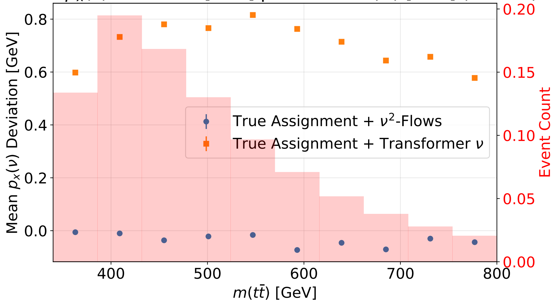
Mean p_x(\nu) Deviation [GeV] per Bin vs m(t\bar{t}) [GeV] (95% CI)
