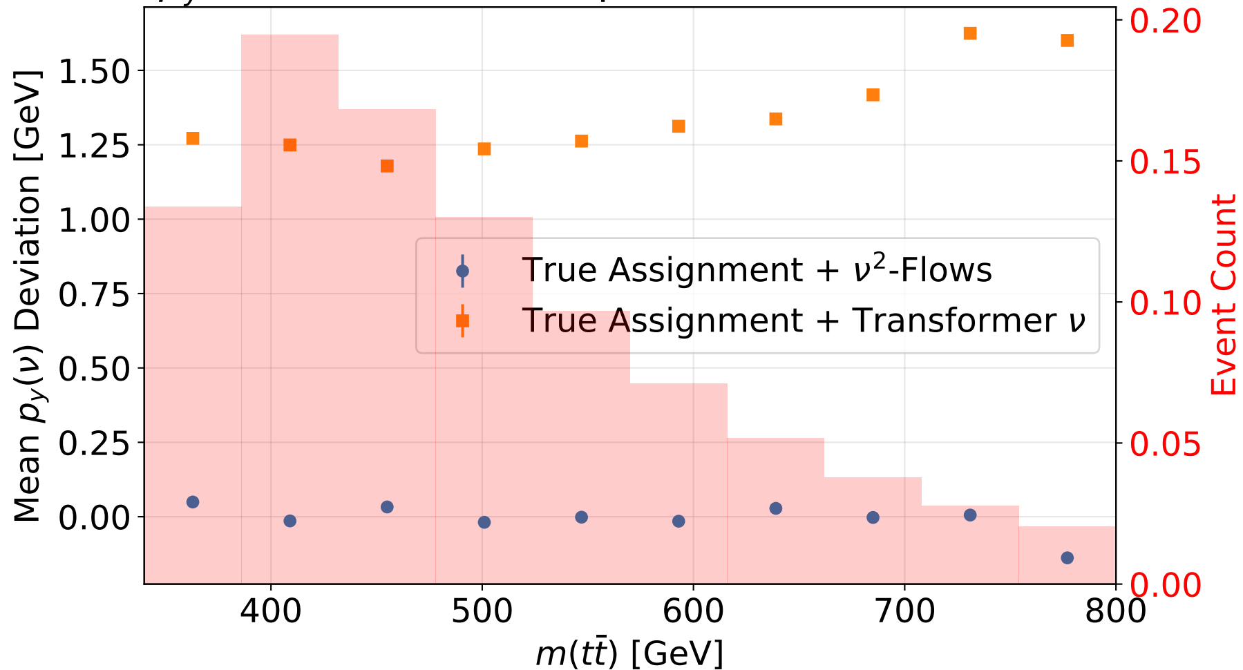
Mean p_y(\nu) Deviation [GeV] per Bin vs m(t\bar{t}) [GeV] (95% CI)
