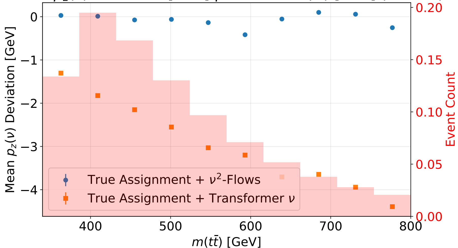
Mean p_z(\nu) Deviation [GeV] per Bin vs m(t\bar{t}) [GeV] (95% CI)
