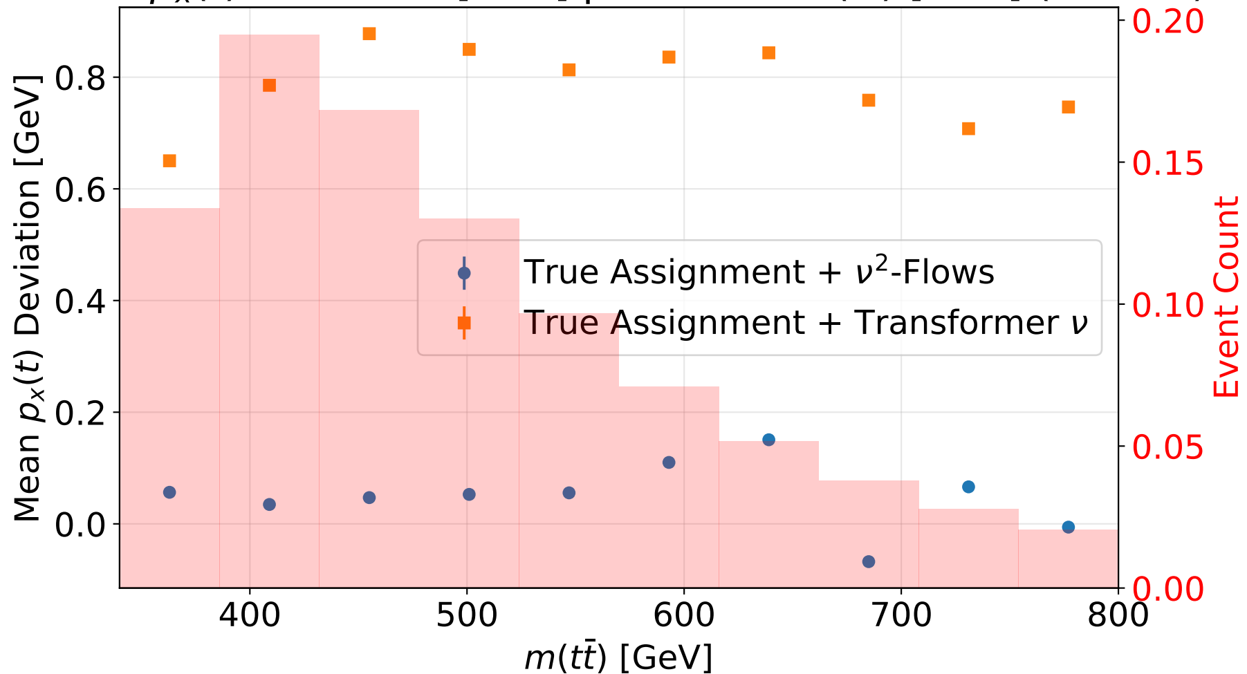
Mean p_x(t) Deviation [GeV] per Bin vs m(t\bar{t}) [GeV] (95% CI)
