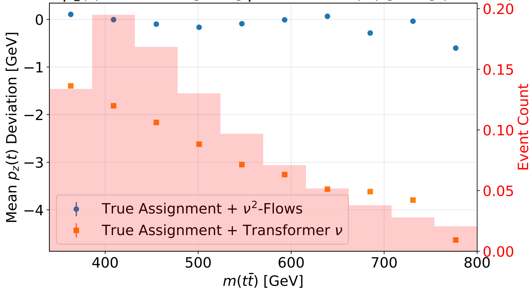
Mean p_z(t) Deviation [GeV] per Bin vs m(t\bar{t}) [GeV] (95% CI)
