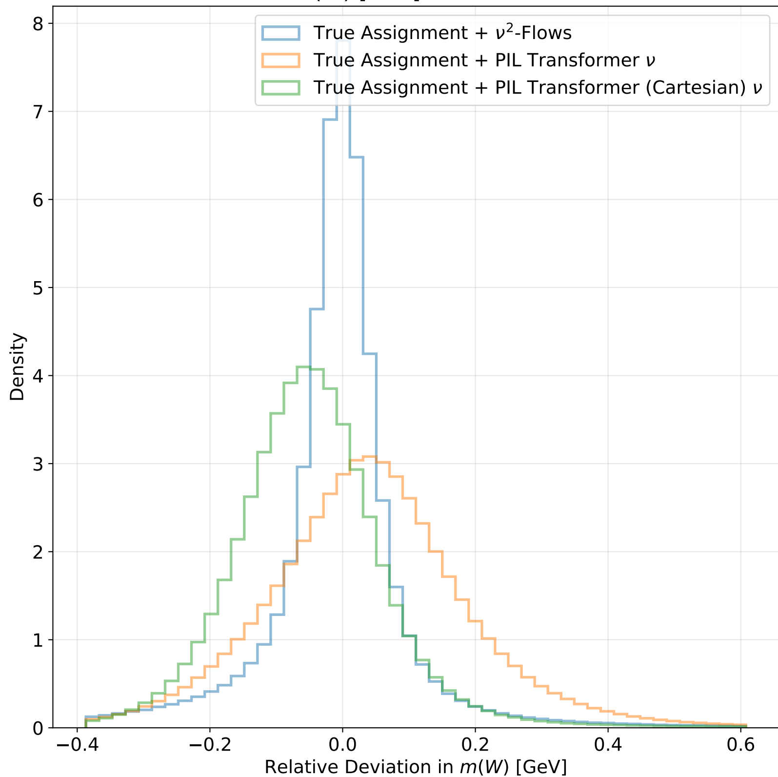
Relative Deviation in m(W) [GeV] Deviation for all Reconstructors
