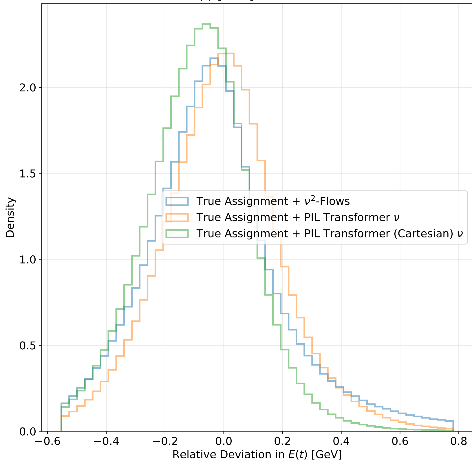
Relative Deviation in E(t) [GeV] Deviation for all Reconstructors
