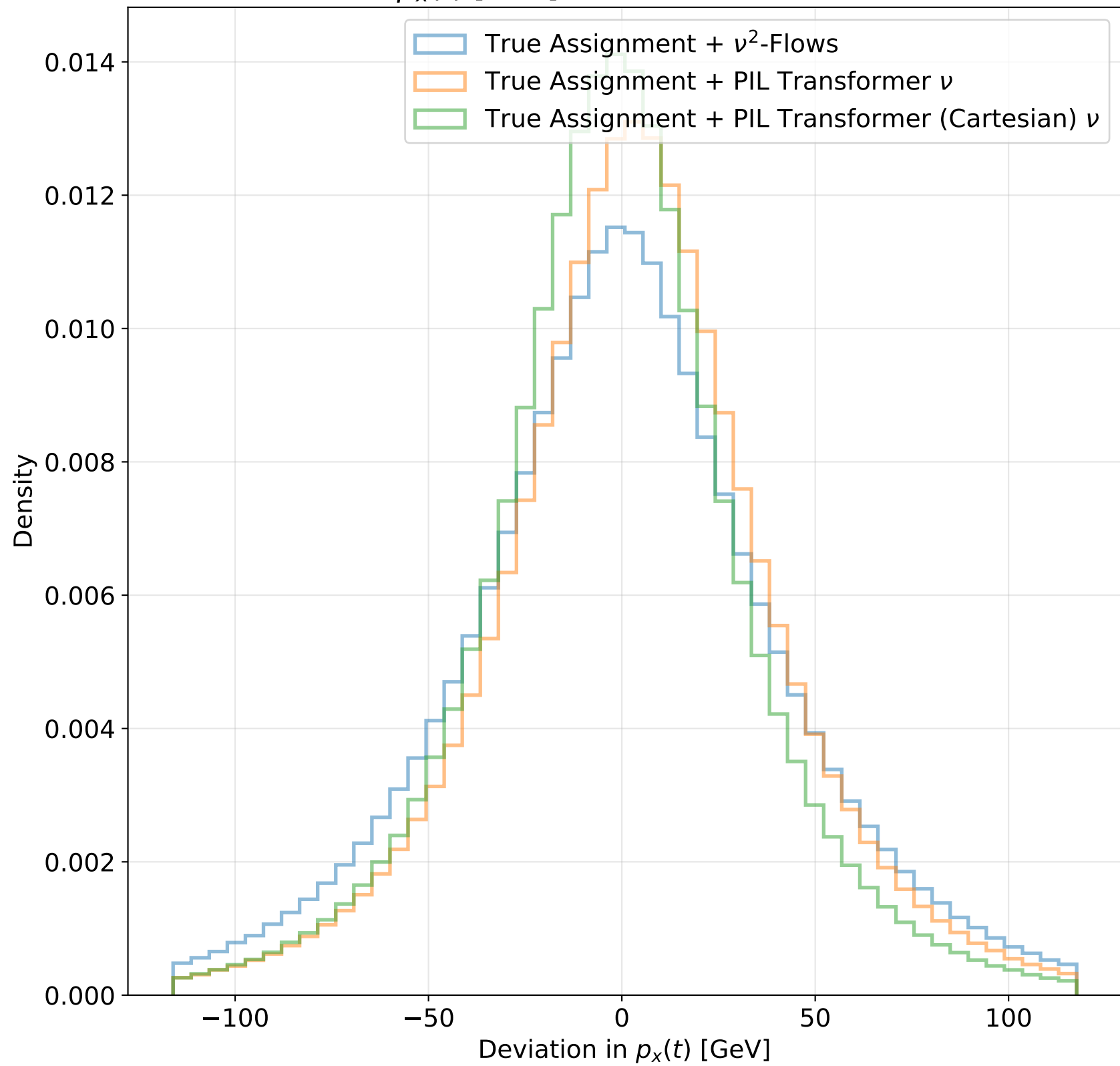
Deviation in p_x(t) [GeV] Deviation for all Reconstructors
