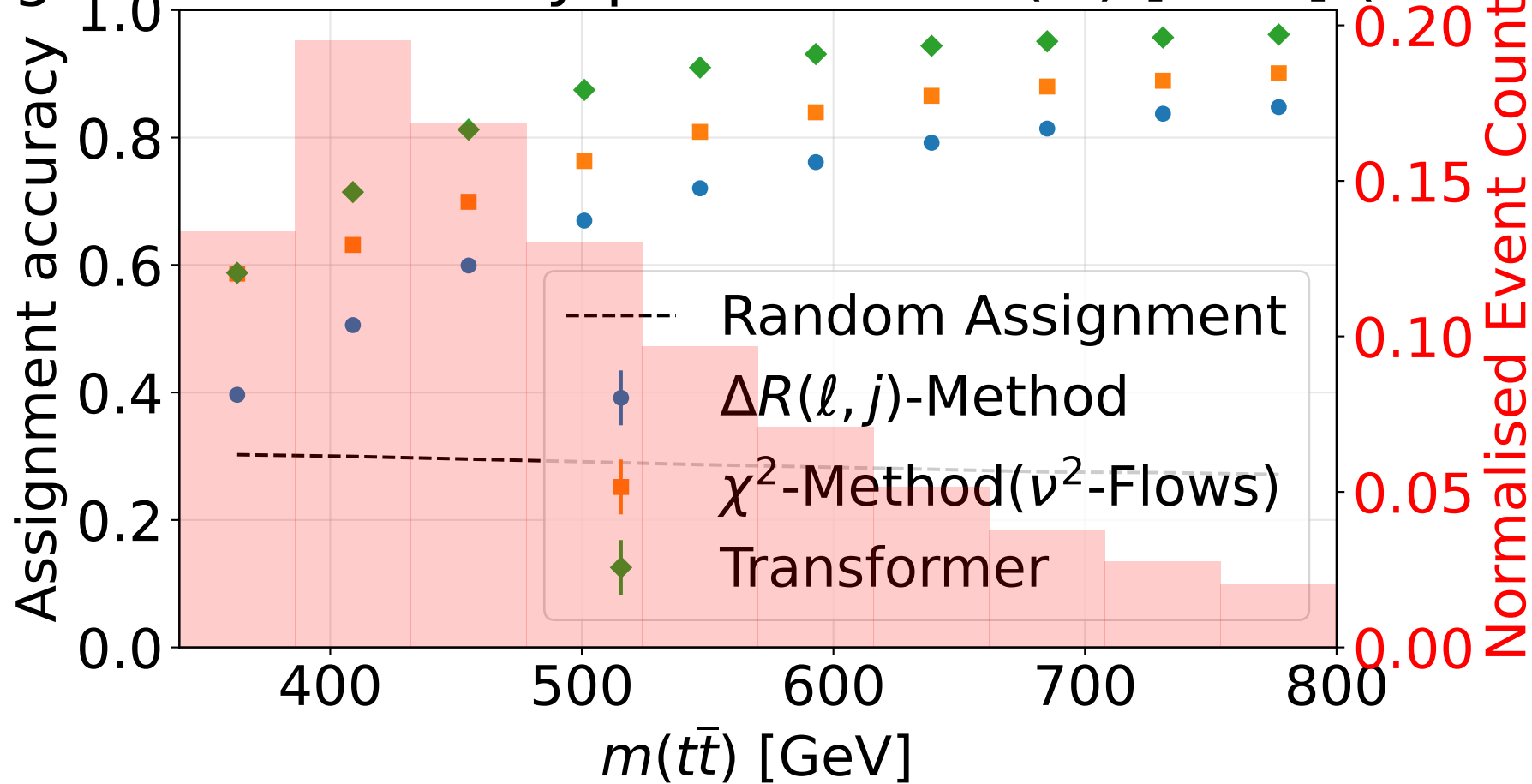
Assignment accuracy per Bin vs m(t\bar{t}) [GeV] (95% CL)
