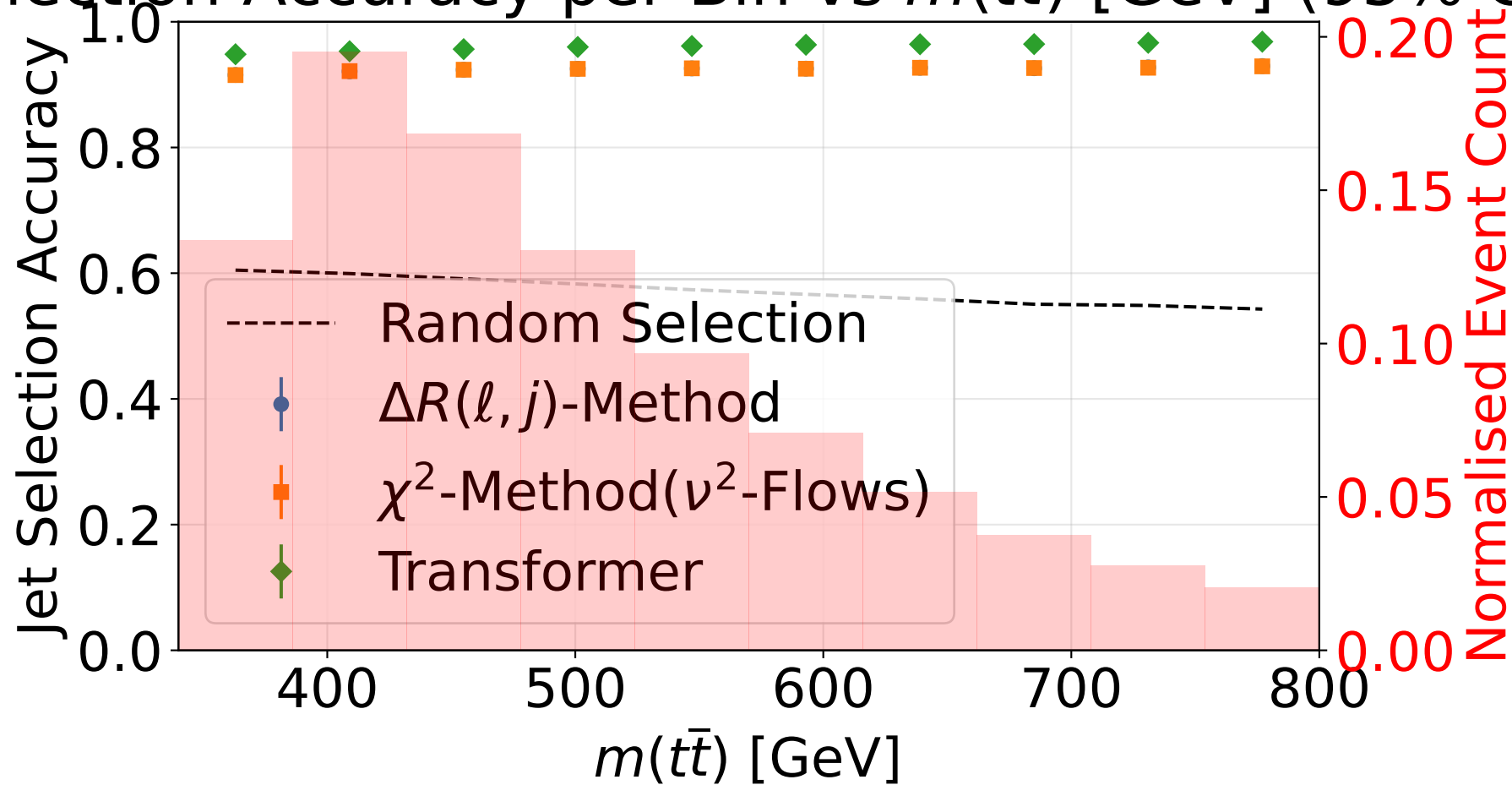
Selection Accuracy per Bin vs m(t\bar{t}) [GeV] (95% CI)
