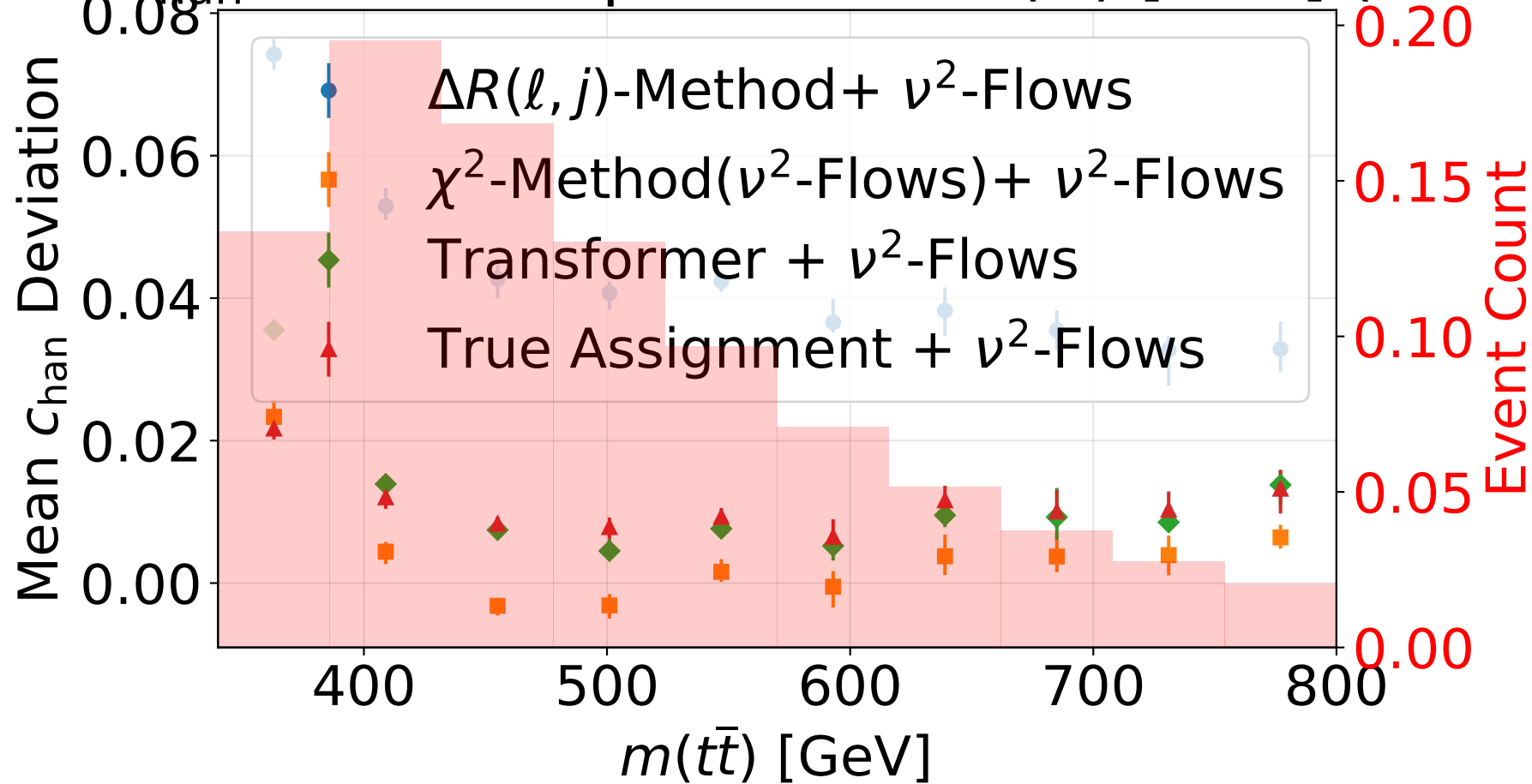
Mean c_{\text{chan}} Deviation per Bin vs m(t\bar{t}) [GeV] (95% CI)
