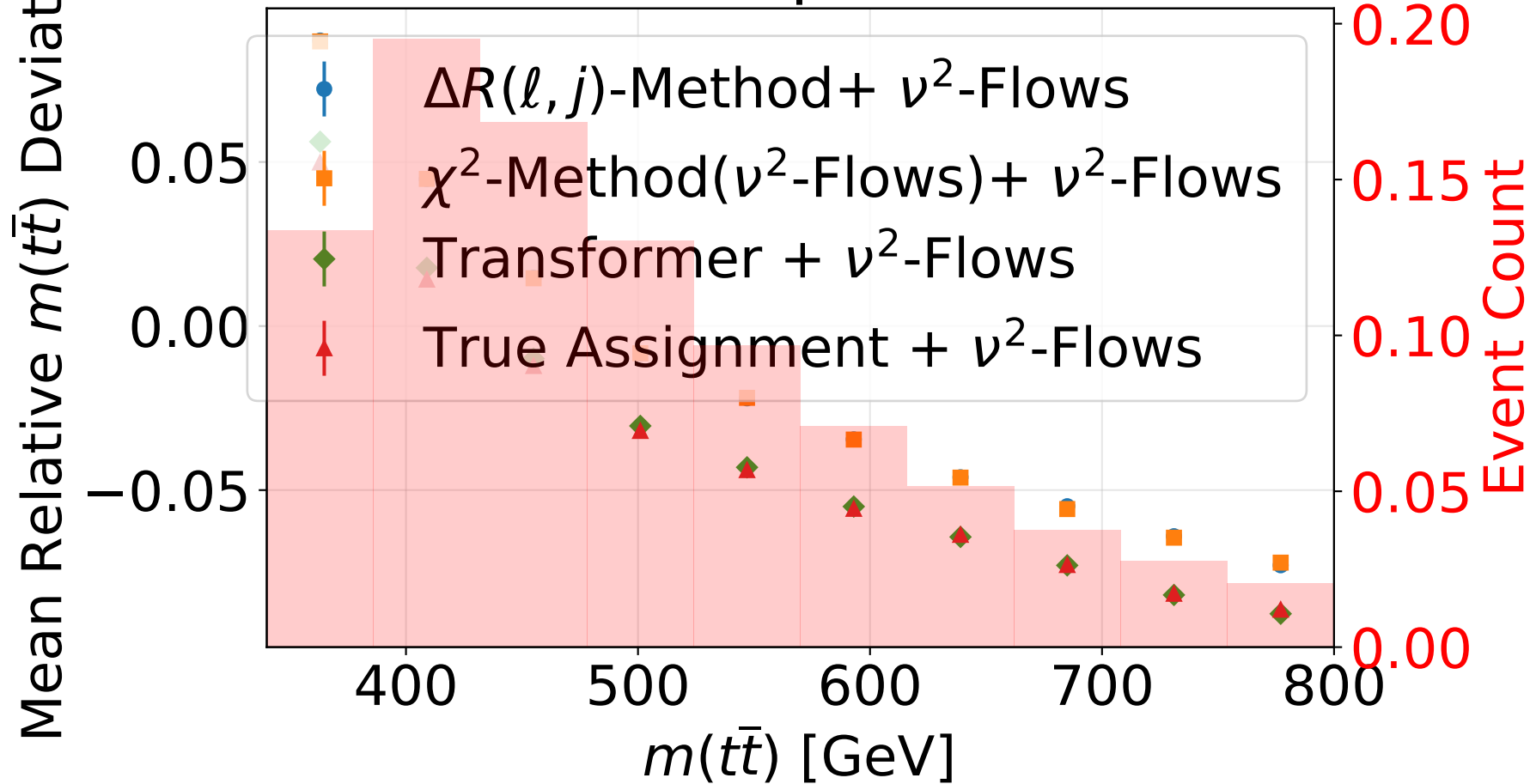
Mean Relative m(t\bar{t}) Deviation per Bin vs m(t\bar{t}) [GeV] (9)
