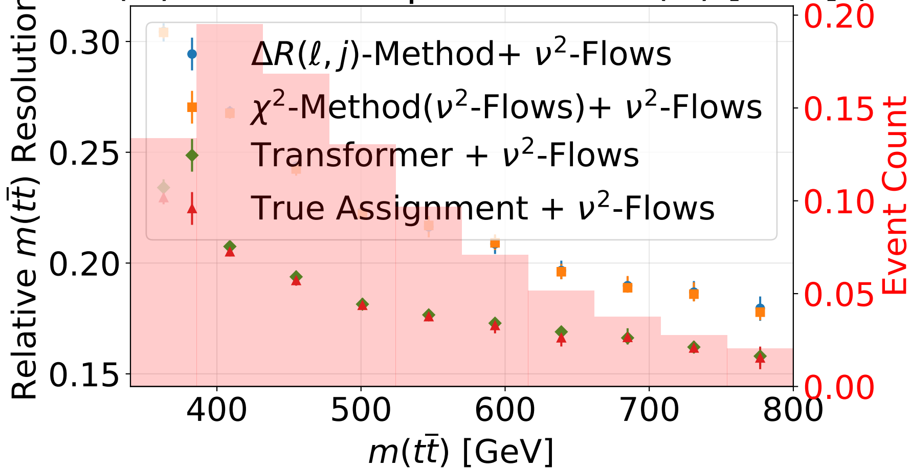
Relative m(t\bar{t}) Resolution per Bin vs m(t\bar{t}) [GeV] (95%)
