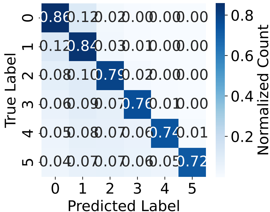
Transformer
