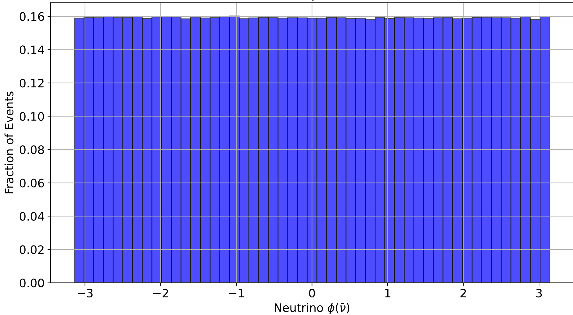
Antineutrino \phi Distribution
