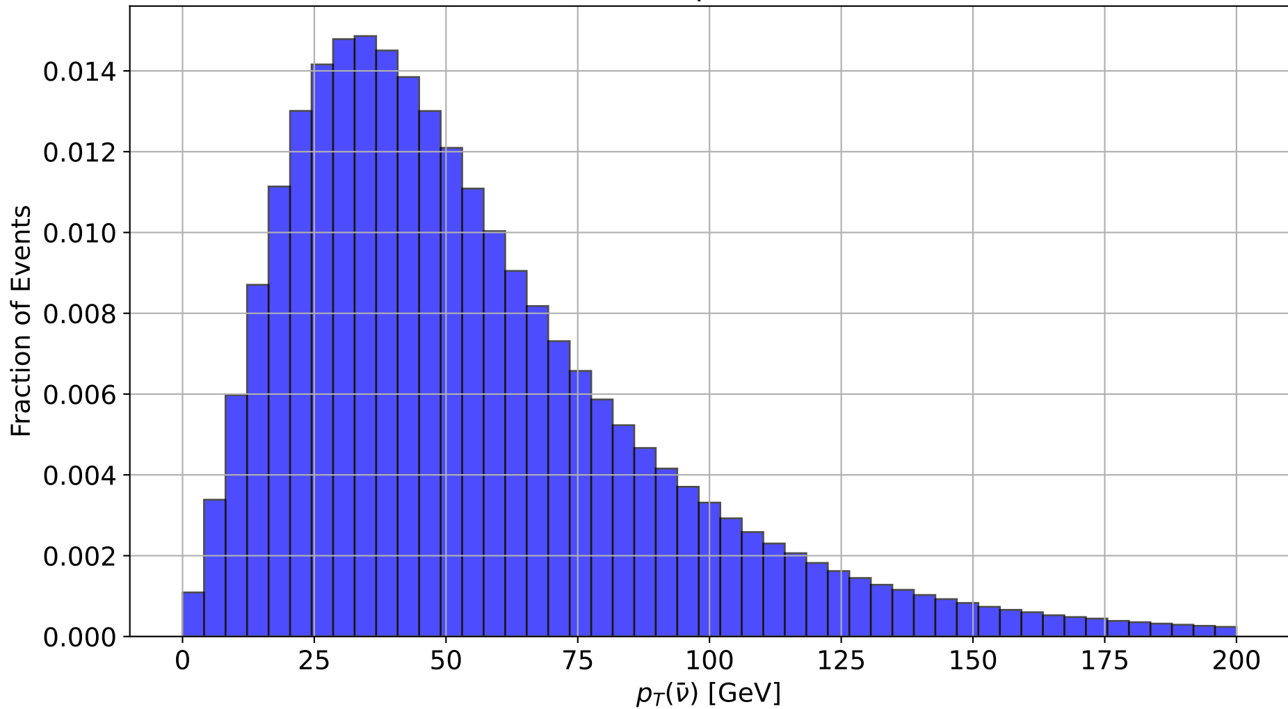
Antineutrino p_T Distribution
