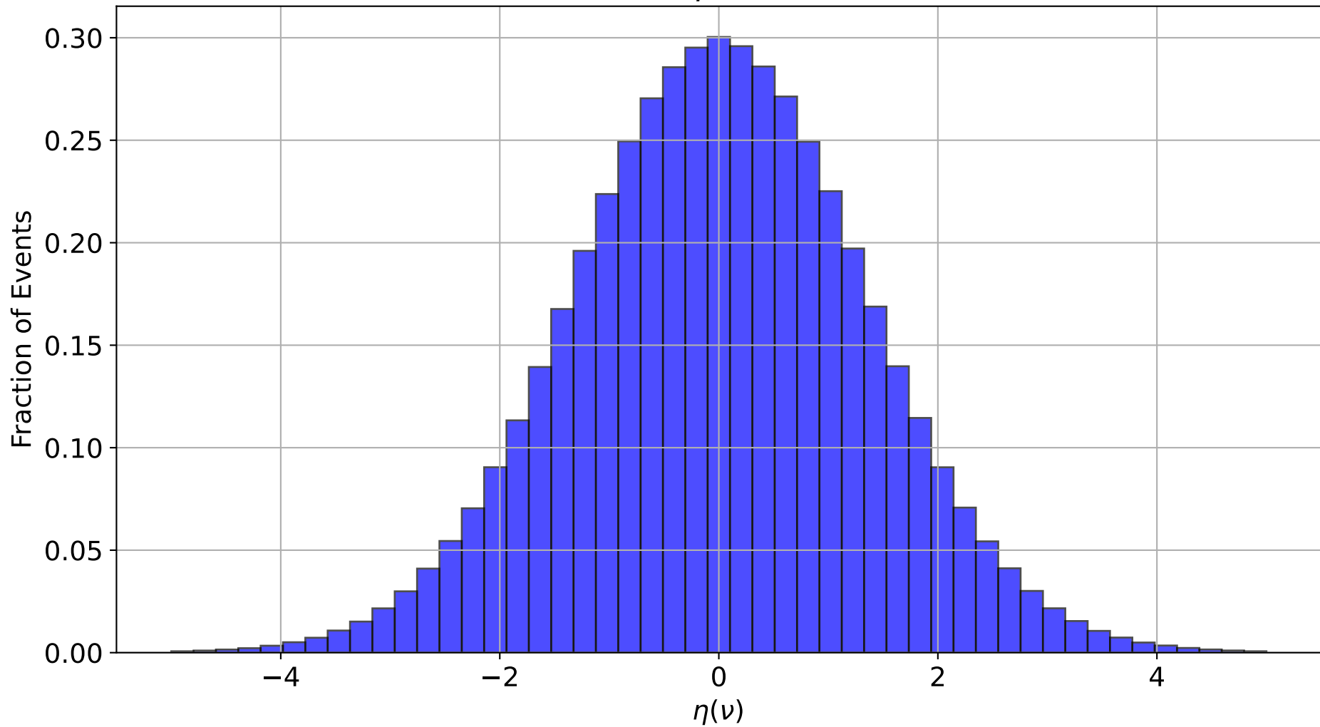
Neutrino \eta Distribution
