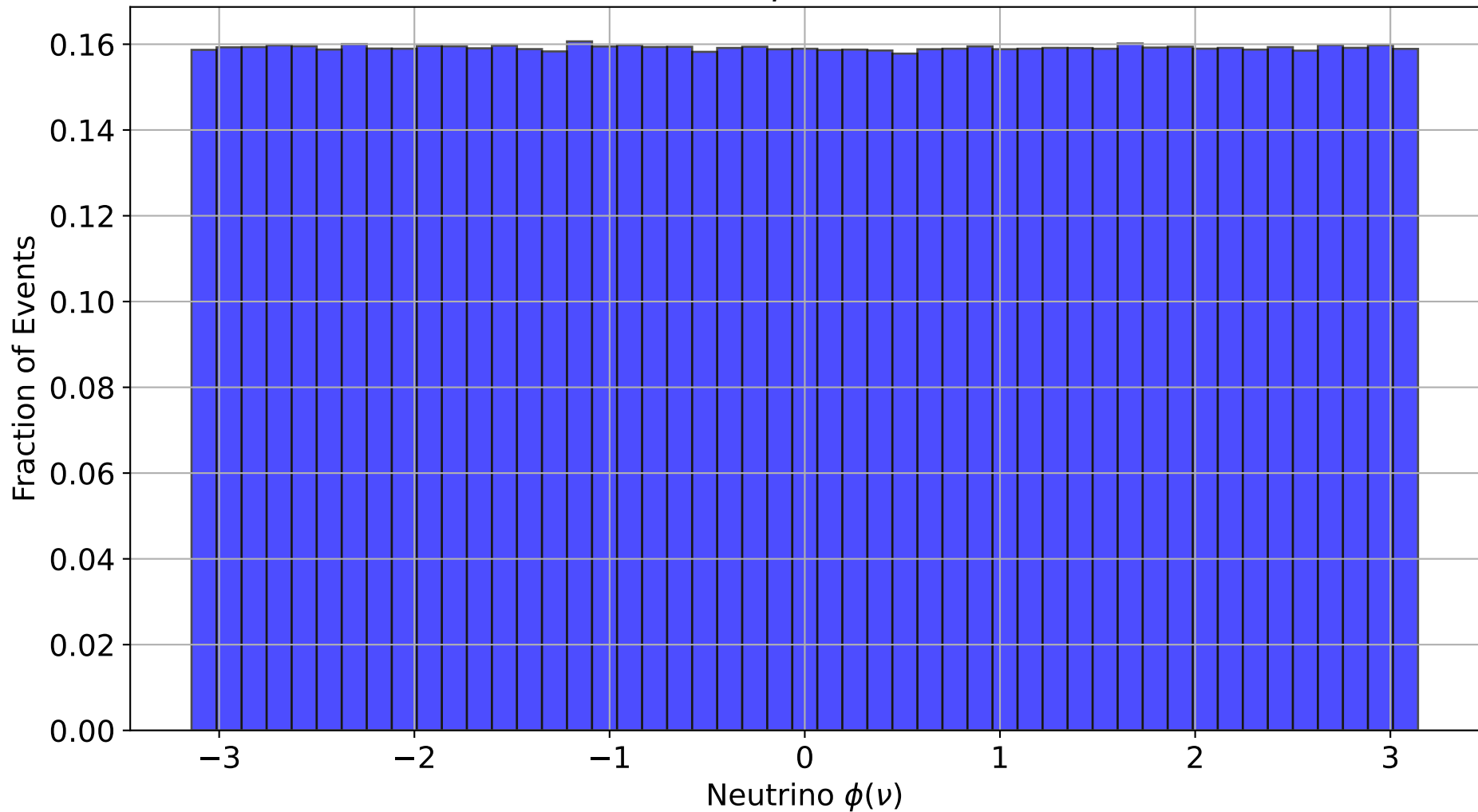
Neutrino \phi Distribution
