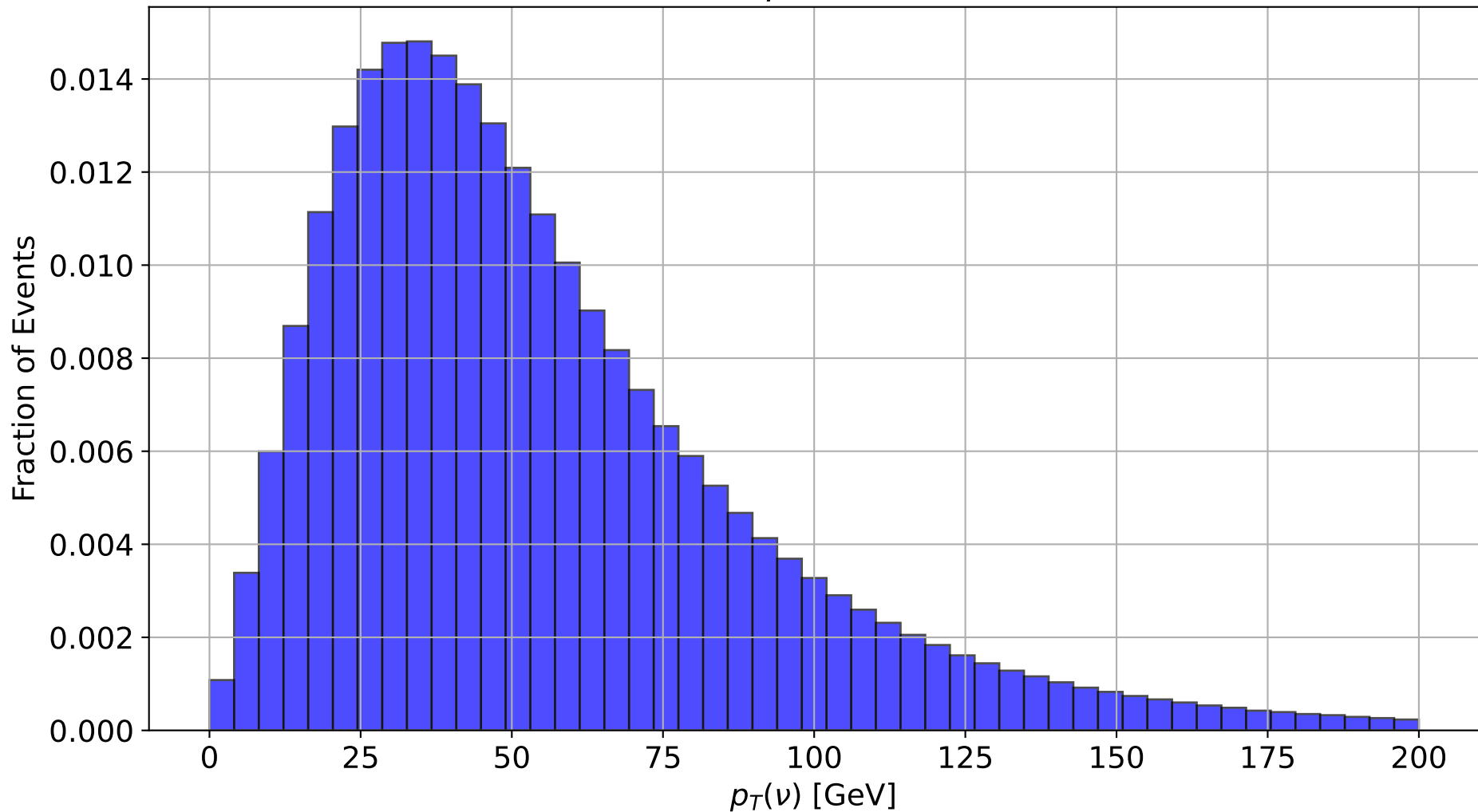
Neutrino p_T Distribution
