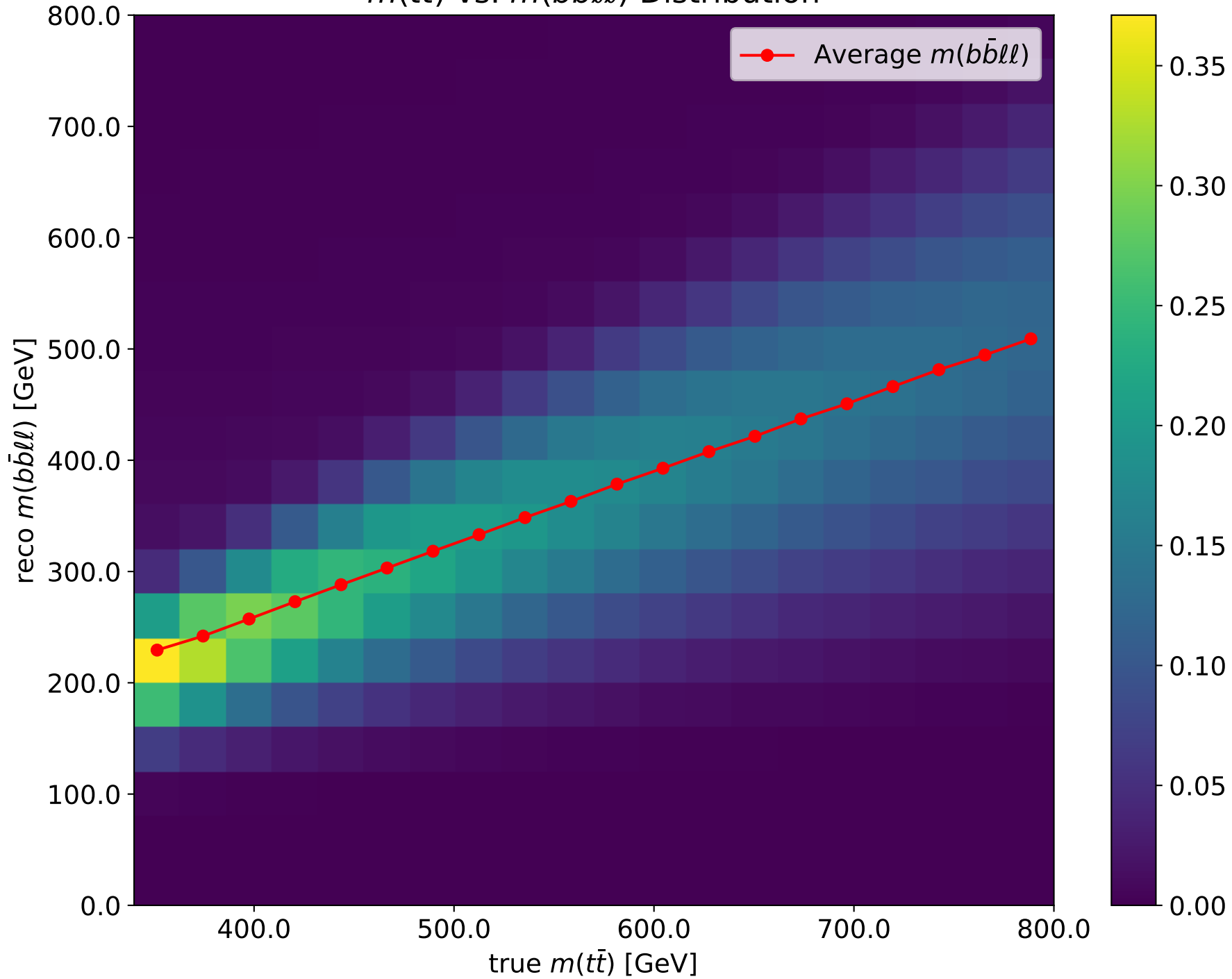
m(t\bar{t}) vs. m(b\bar{b}l\bar{l}) Distribution
