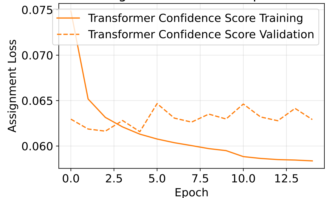
Assignment Loss Over Epochs
