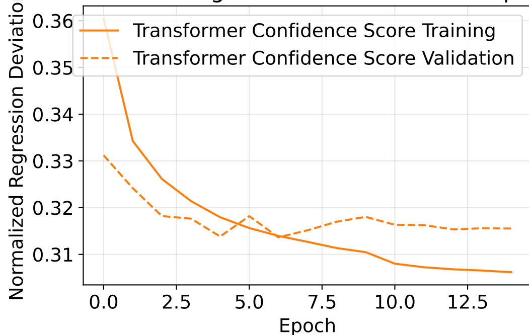
Normalized Regression Deviation Over Epochs
