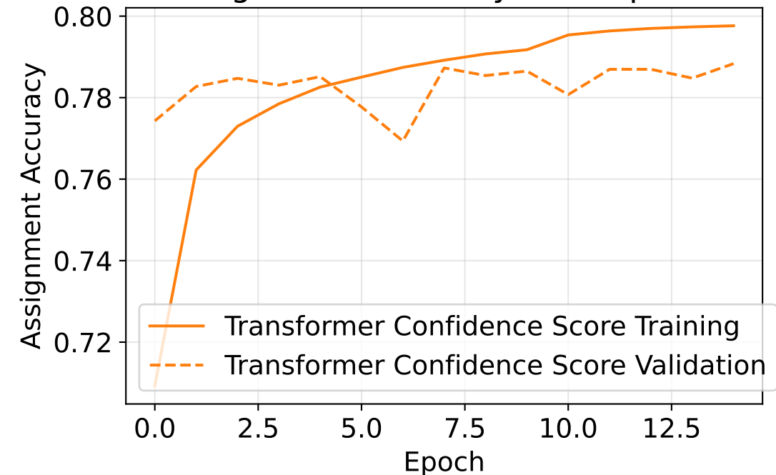
Assignment Accuracy Over Epochs
