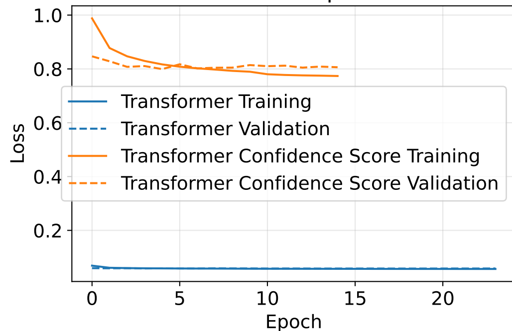
Loss Over Epochs
