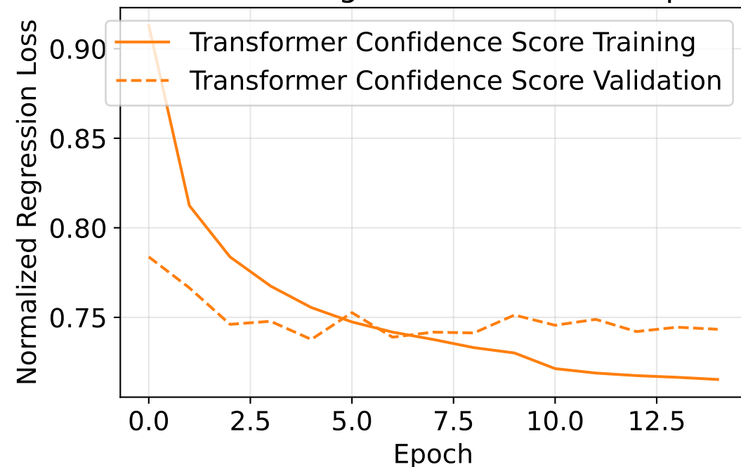
Normalized Regression Loss Over Epochs
