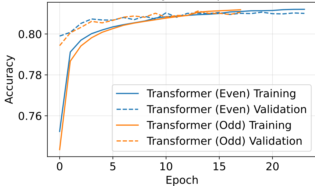
Accuracy Over Epochs
