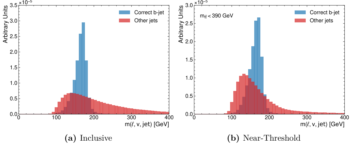
Figure A.7.: Distribution of m(\ell, \nu, j) for correct and incorrect pairing of jets and leptons. Evaluated on the full sample in (a) and near-threshold in (b).
