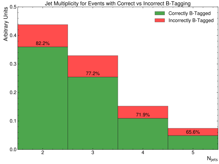
Figure A.4.: This plot shows the b-tagging performance for different numbers of jets in the event. For each jet multiplicity, the number of events, with only jets from top-decays being b-tagged
