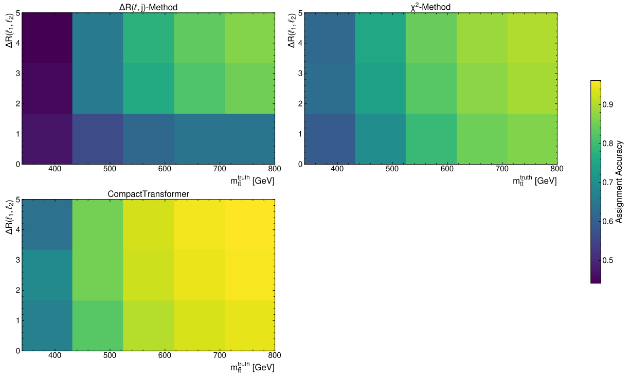
Figure A.9.: Assignment accuracy binned with respect to parton-level m(t\bar{t}) and \Delta R(\ell_1, \ell_2) .
