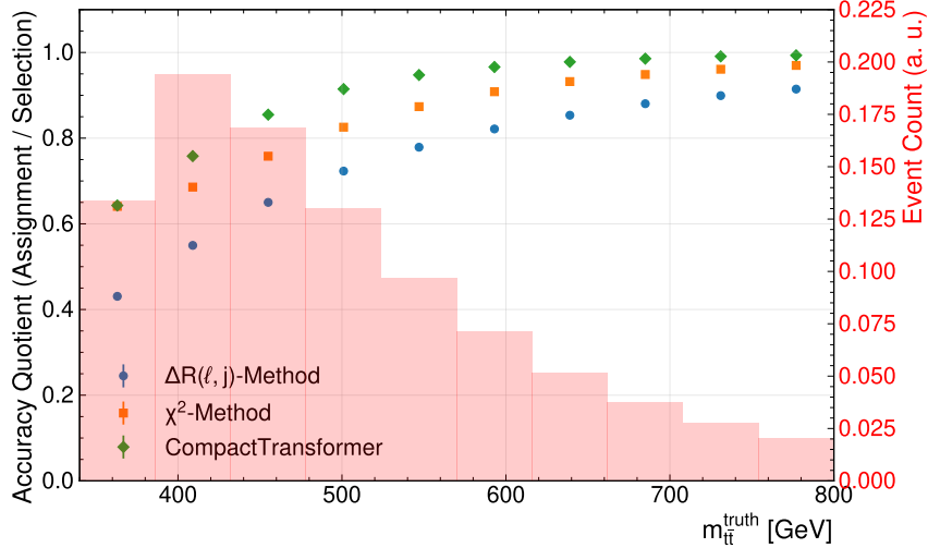
Figure 7.3.: Quotient of assignment and selection accuracy computed in bins of the parton-level m(t\bar{t}) .
