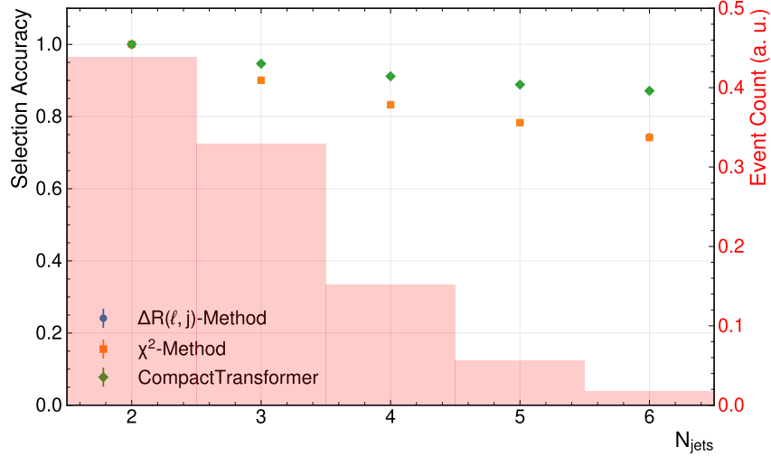
Figure A.8.: Selection accuracy as a function of the number of jets in the event for different reconstruction methods. The background histograms show of the distribution of events as a function of the number of jets. The uncertainties represent the statistical variations in the evaluation dataset.
